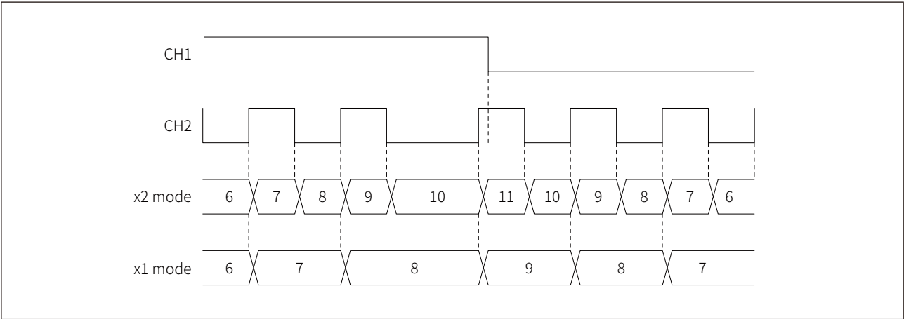
Figure 16-30 Example of clock + direction encoder mode counting
