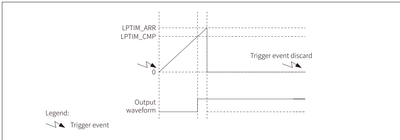
Figure 15-4 LPTIM single set waveform
