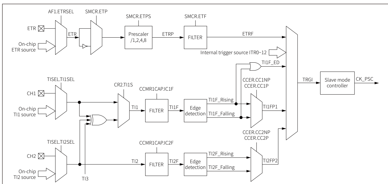
Figure 16-21 External clock mode 1 connection diagram
