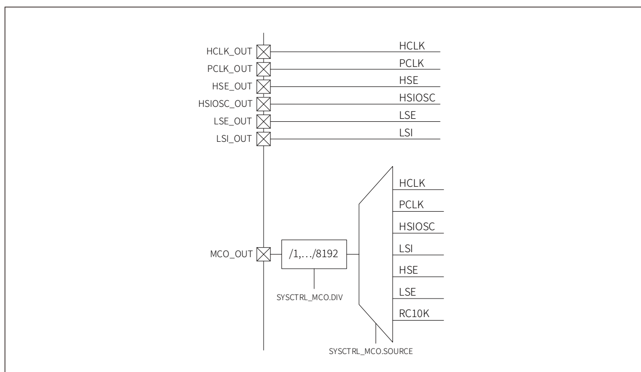
Figure 4-5 Clock output
