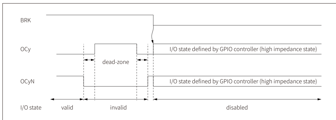
Figure 17-50 Output behavior in response to braking event BRK (OSSl = 0)
