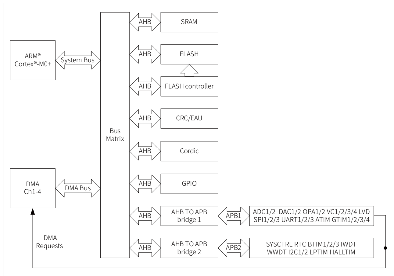
Figure 2-1 System architecture
