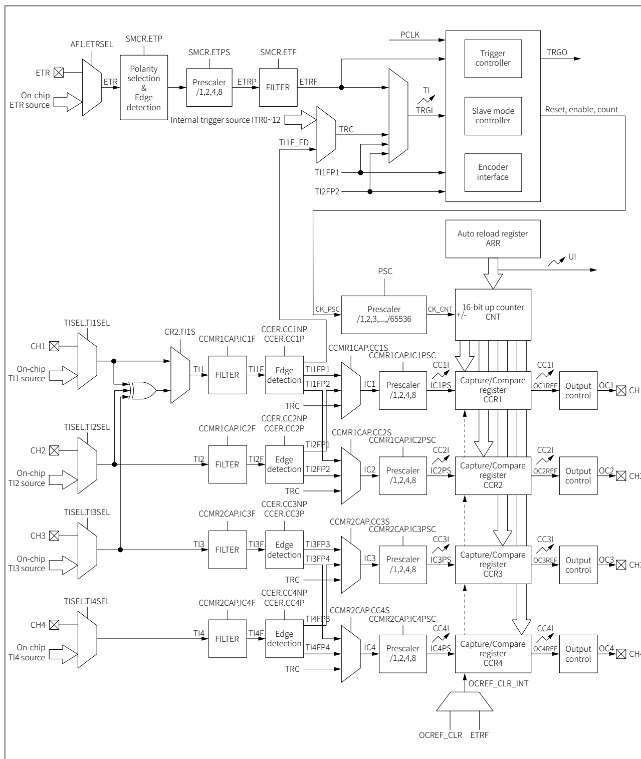
Figure 16-1 GTIM functional block diagram
