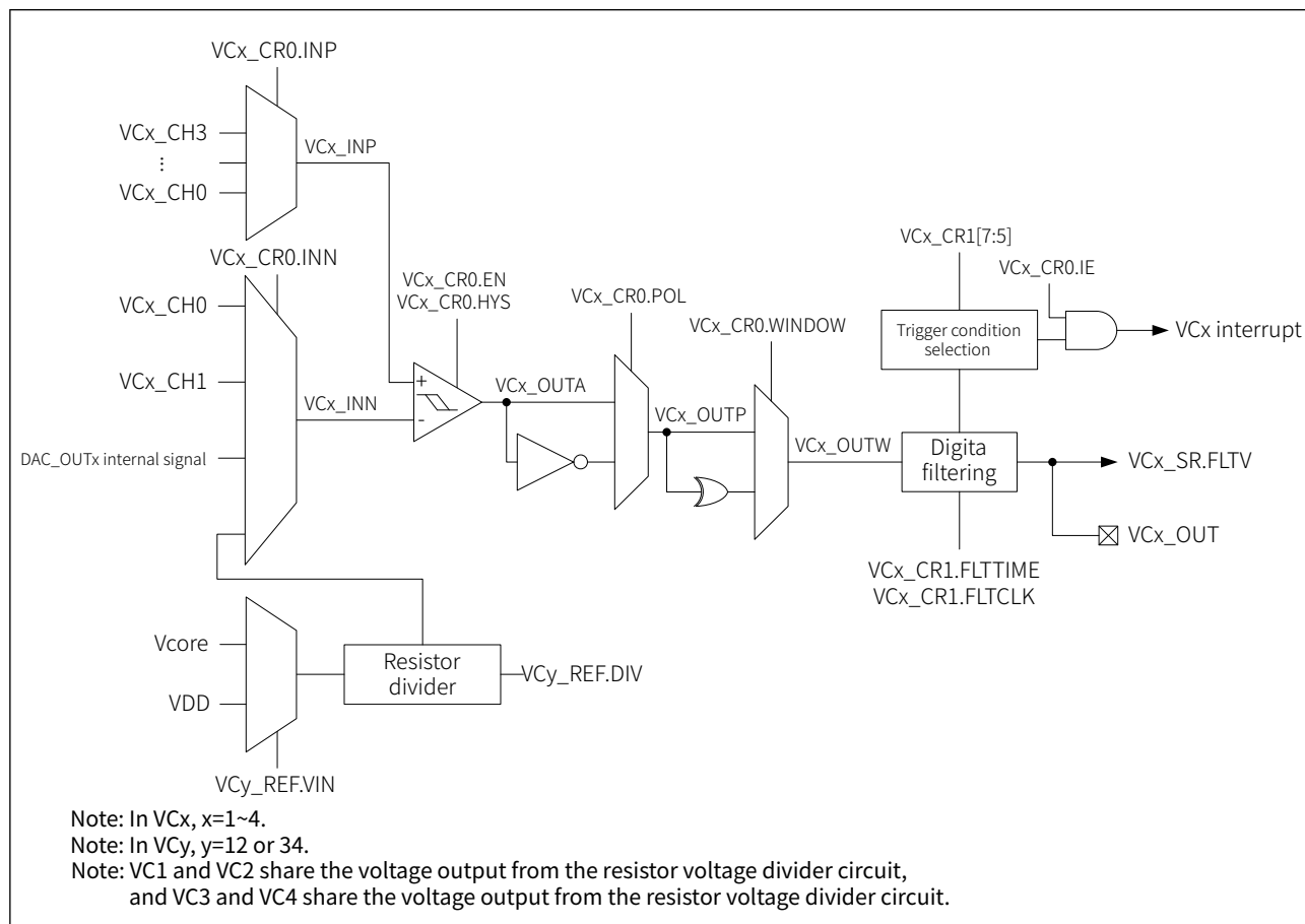
Figure 27-1 VC functional block diagram
