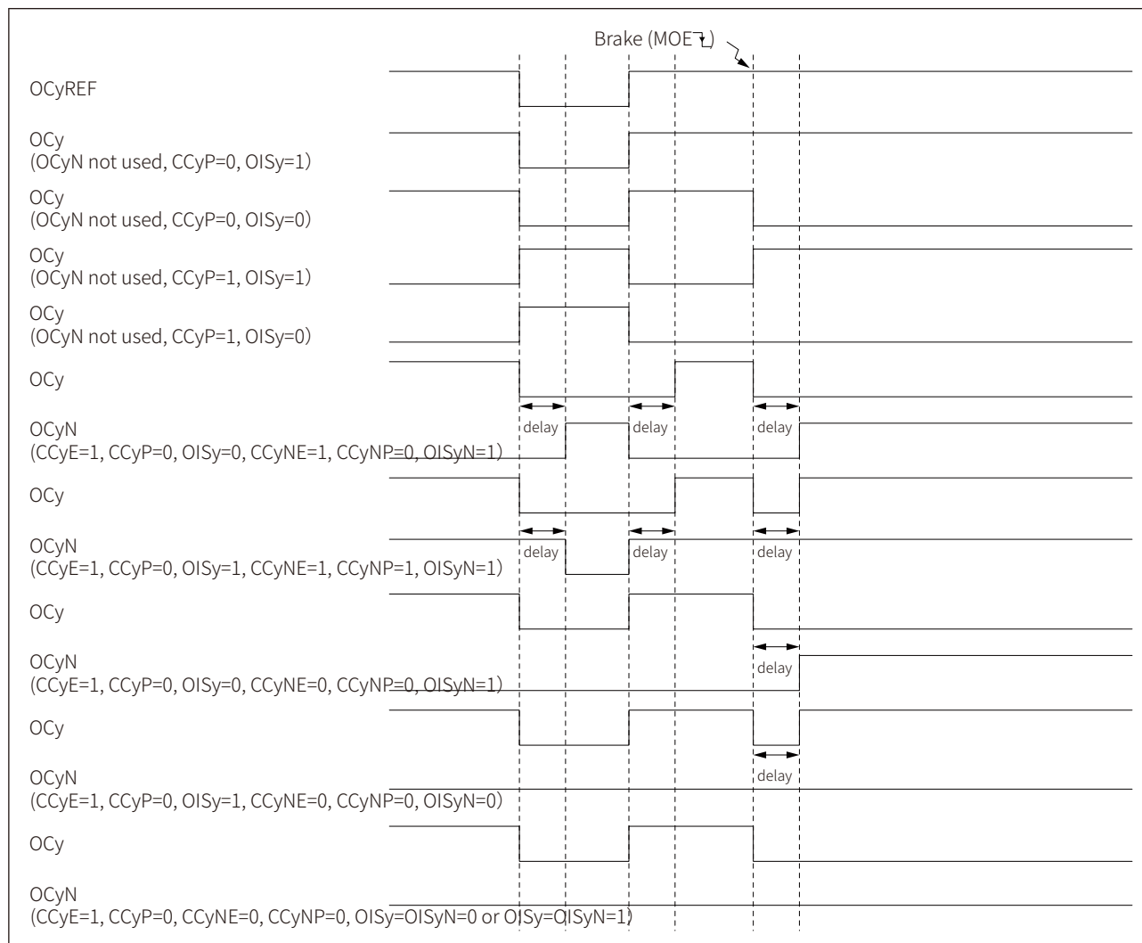
Figure 17-50 Output behavior in response to braking event BRK (OSSl = 0)
