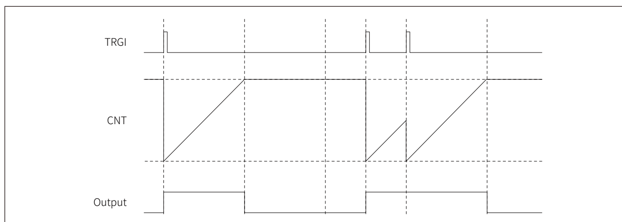
Figure 17-52 Example of retriggerable single pulse mode 2
