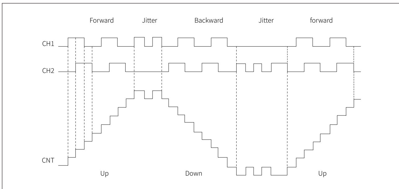
Figure 16-28 Example of quadrature encoder mode-x4 mode operation
