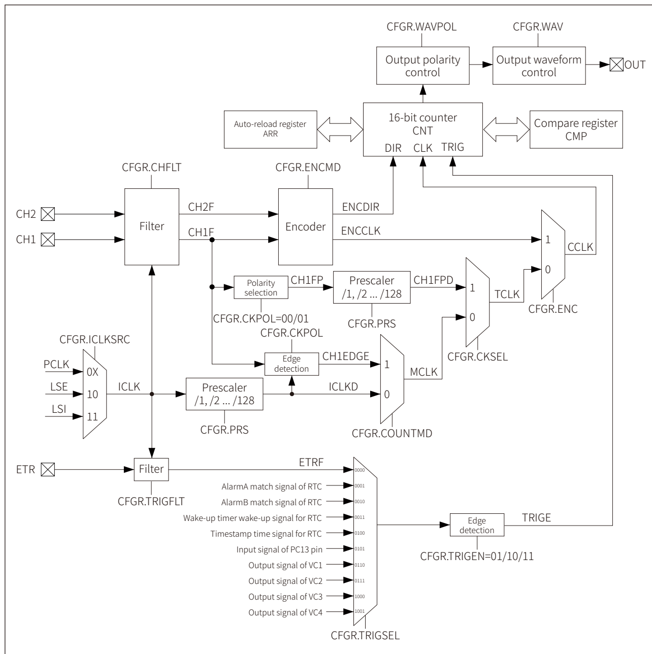
Figure 15-1 LPTIM functional block diagram
