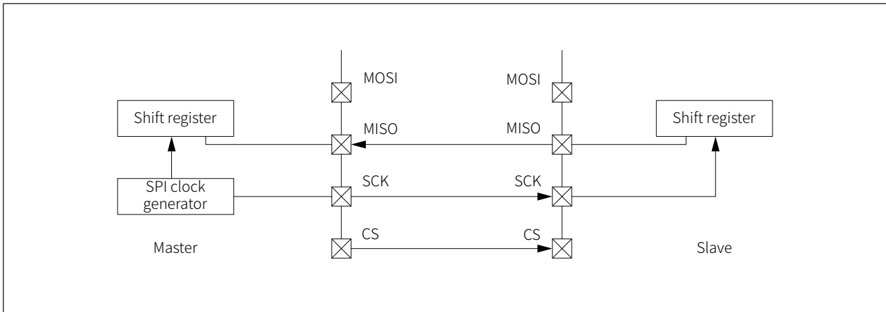
Figure 22-9 Master single receiving, slave single transmitting mode
