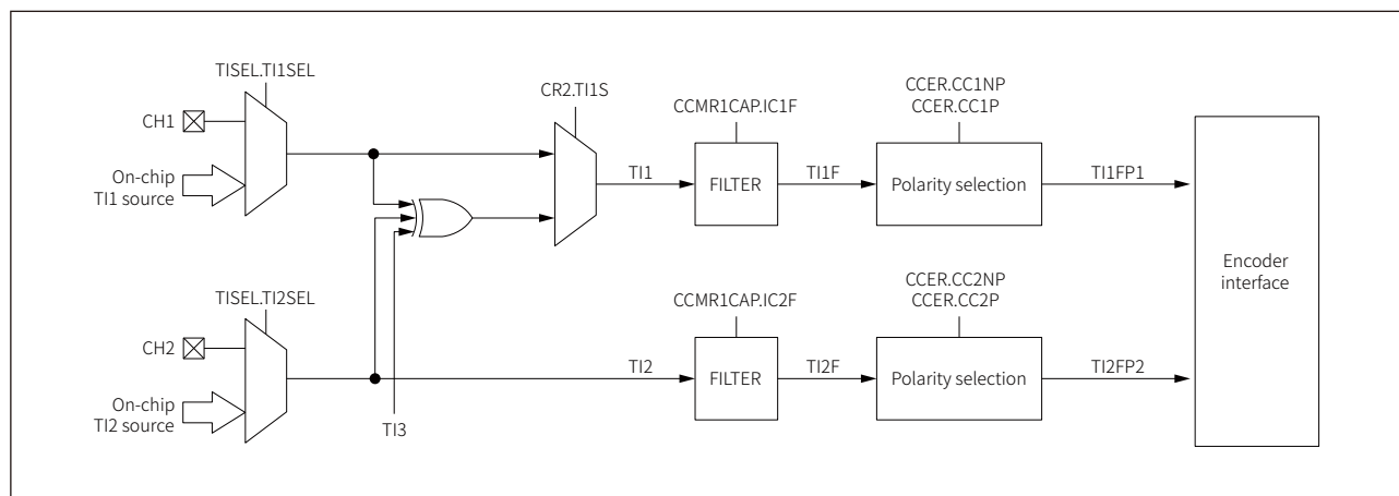
Figure 16-27 Encoder mode block diagram
