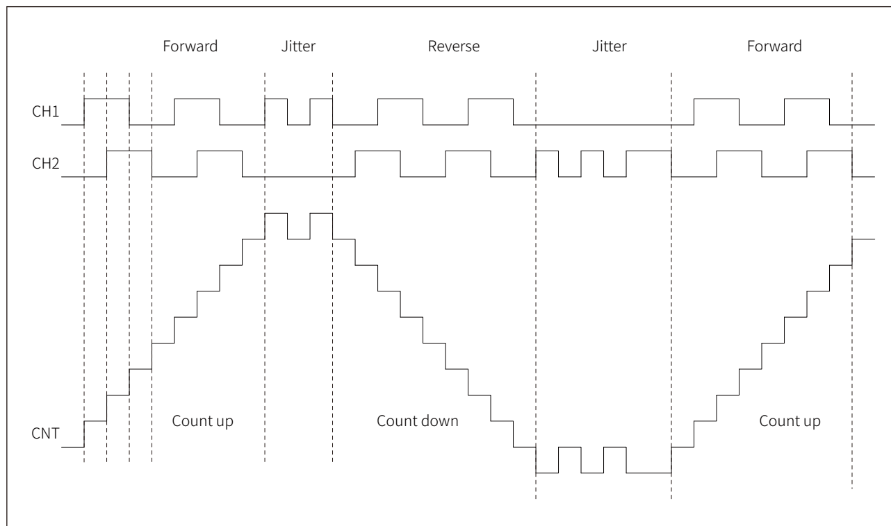
Figure 15-7 Encoder mode count example
