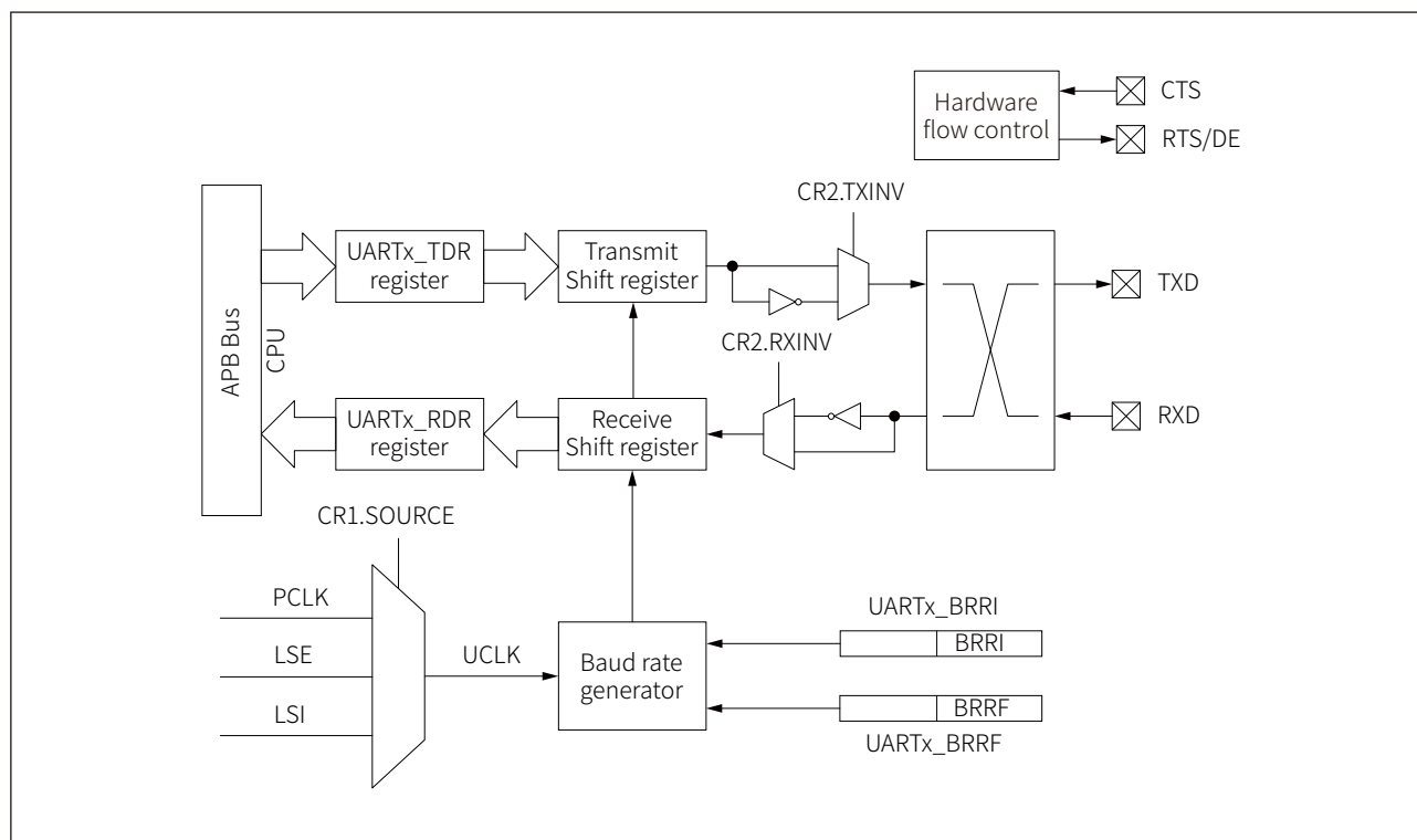
Figure 21-1 UART functional block diagram
