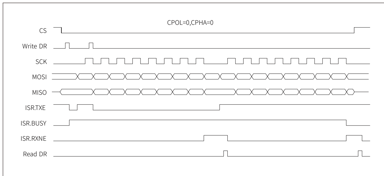
Figure 22-5 Master transmits and receives timing in full-duplex mode (two bytes)
