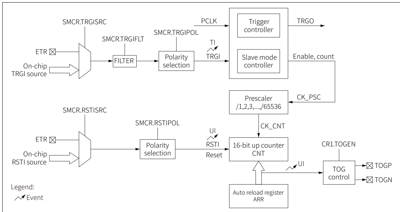
Figure 14-1 BTIM functional block diagram
