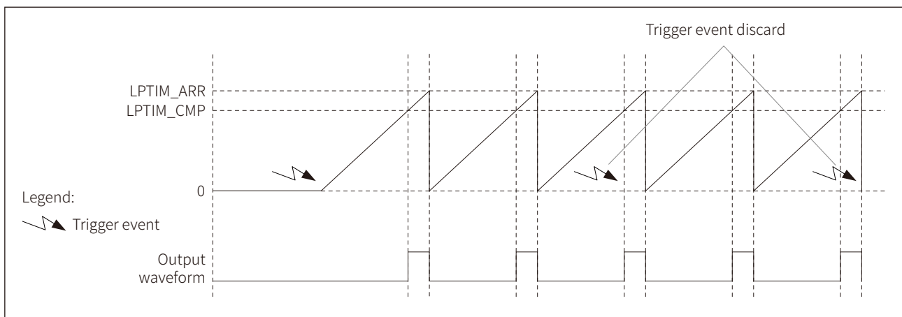
Figure 15-5 LPTIM continuous mode
