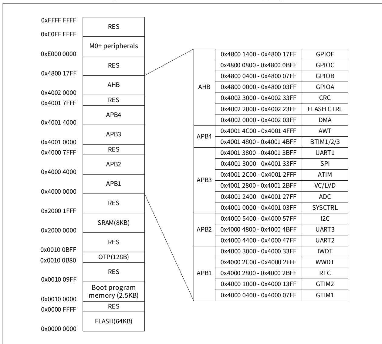
Figure 6-1 CW32L031 internal address mapping
