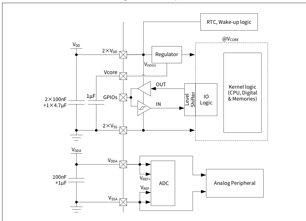
Figure 7-3 Power system
