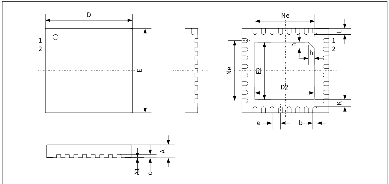
Figure 8-5 QFN32 outline
