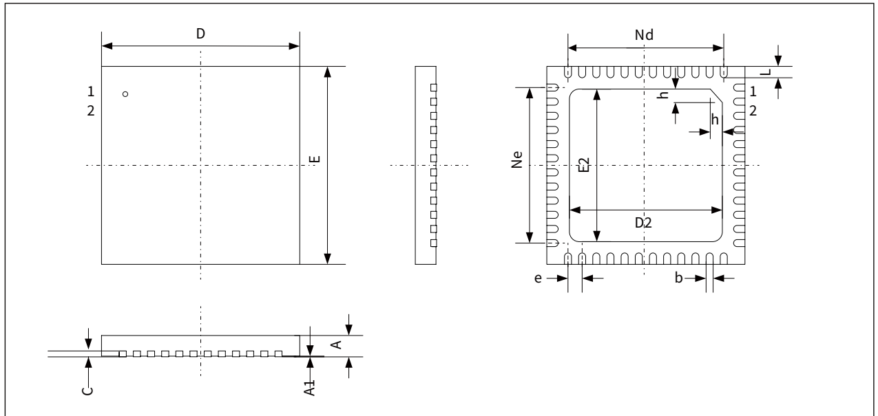
Figure 8-3 QFN48 outline
