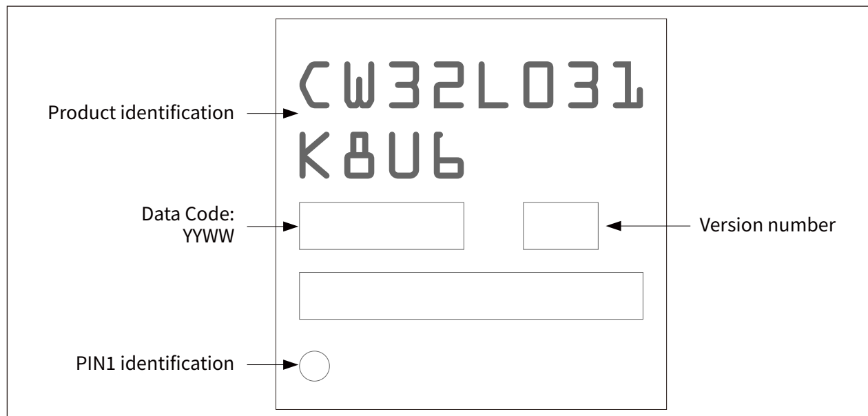
Figure 8-6 QFN32 (5mm x 5mm) topside marking example
