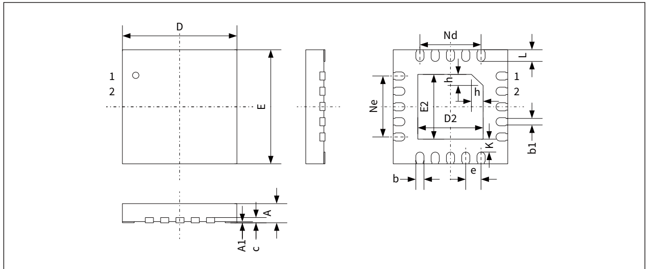
Figure 8-9 QFN20 outline
