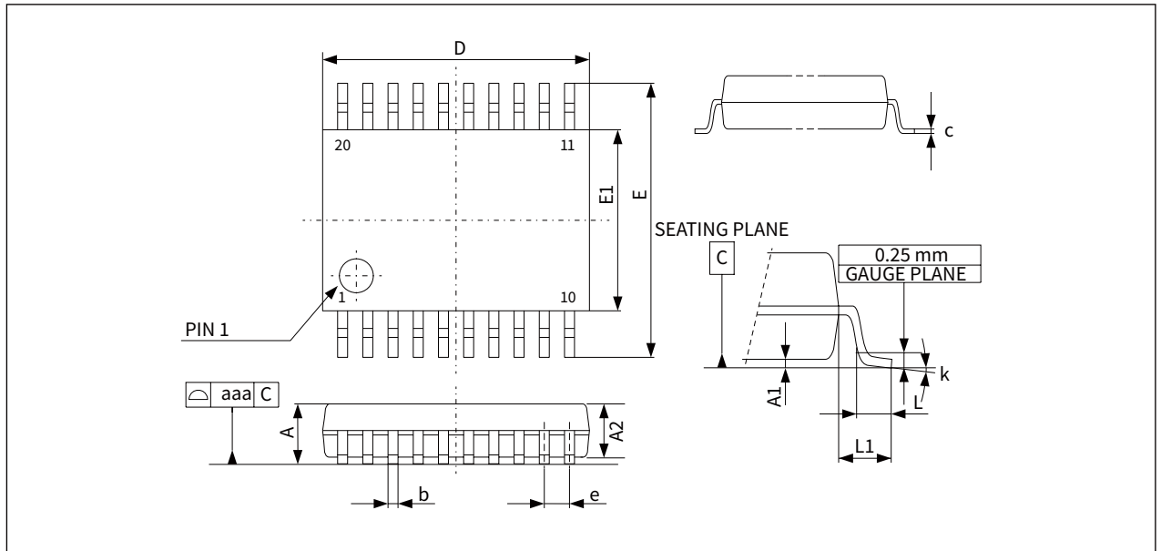
Figure 8-11 TSSOP20 outline
