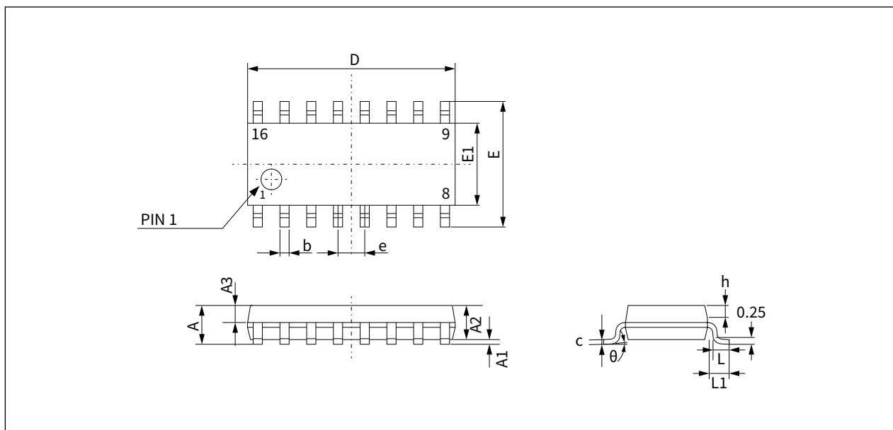
Figure 8-5 SOP16 outline
