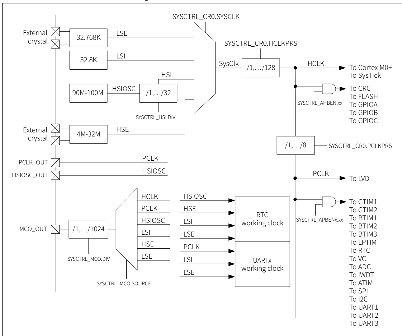
Figure 4-1 Clock tree of CW32L011
