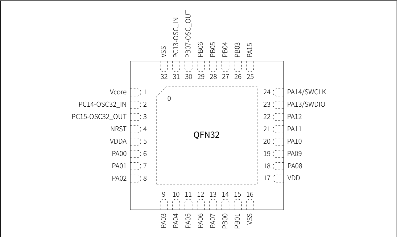
Figure 5-2 QFN32 package pinout (top view)
