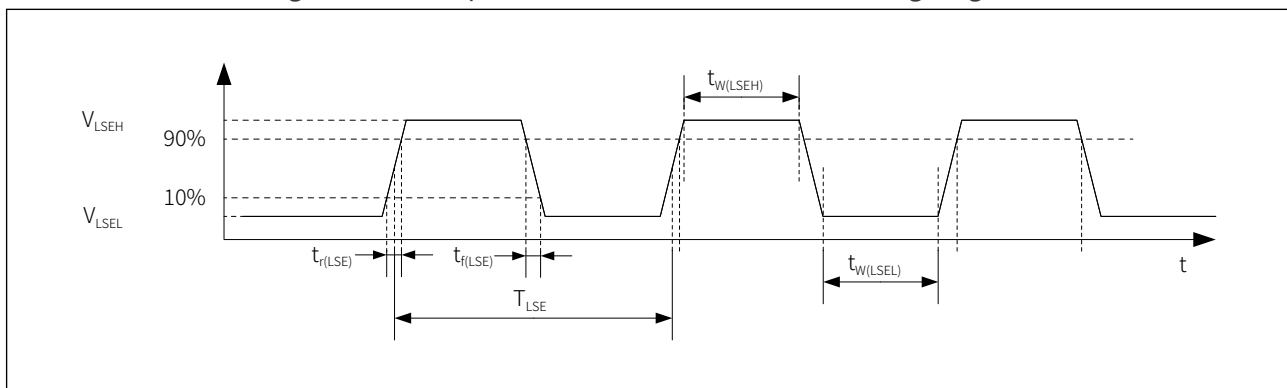
Figure 7-6 Low-speed external clock source AC timing diagram
