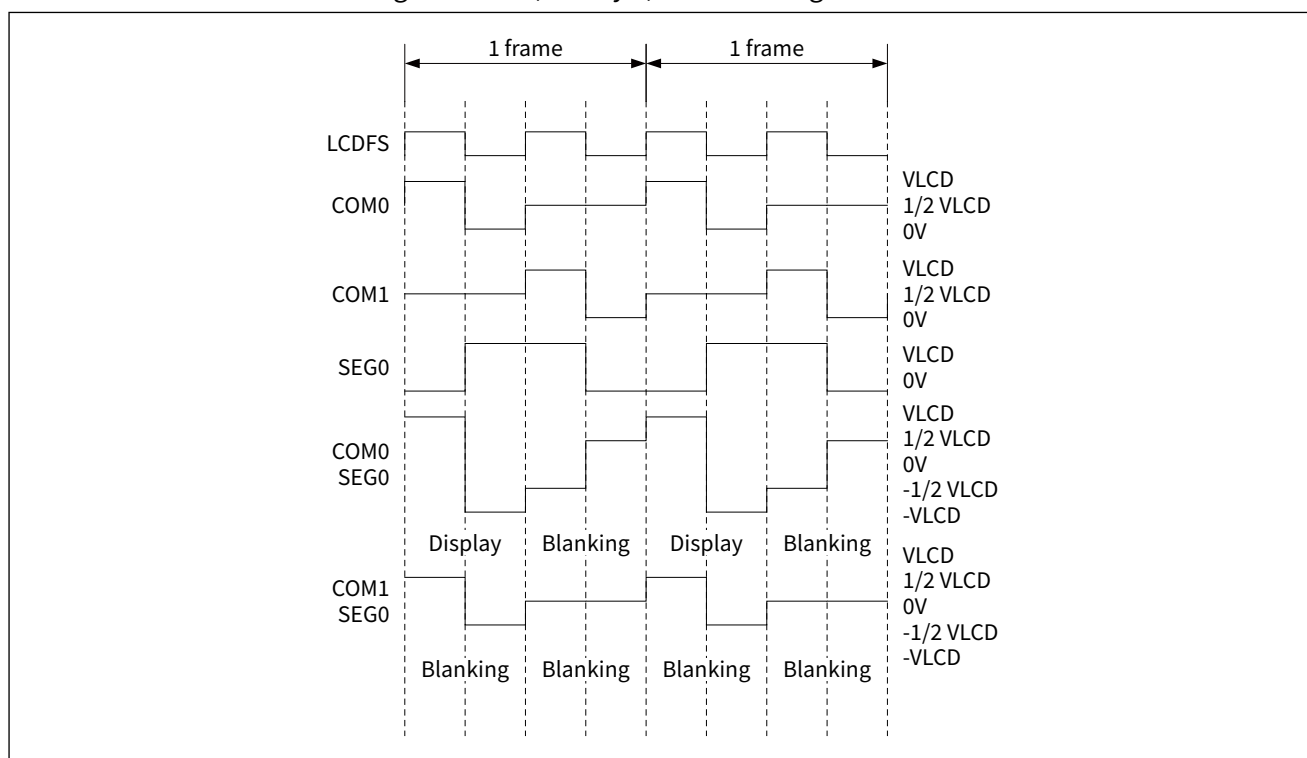
Figure 27-5 1/2 Duty 1/2 Bias driving waveform
