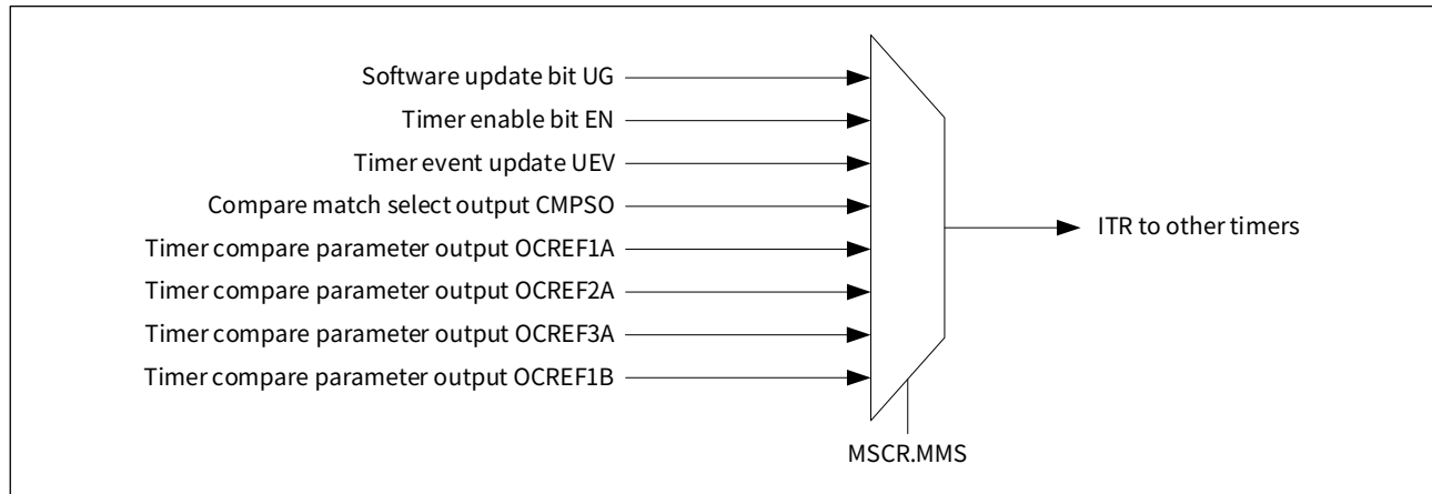
Figure 16-34 ATIM internal cascade ITR
