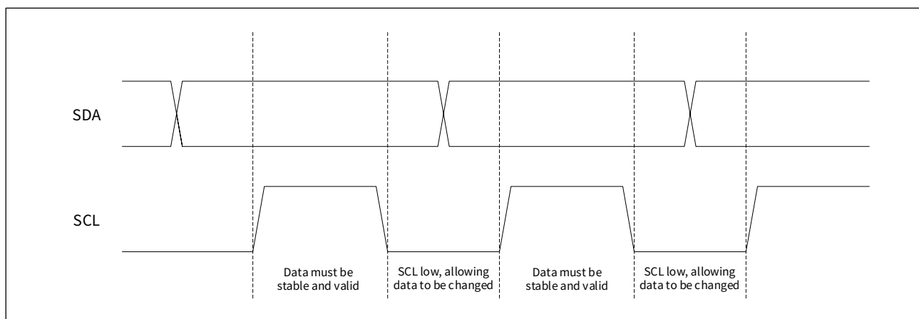
Figure 21-3 Data transmission
