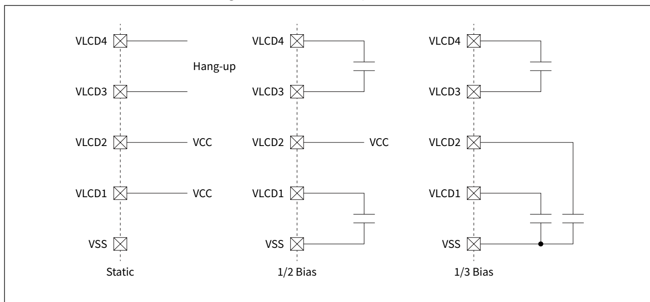
Figure 27-3 External Capacitor Mode
