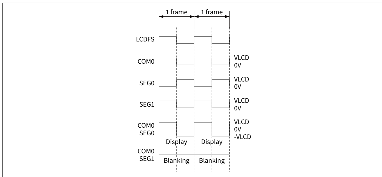
Figure 27-5 1/2 Duty 1/2 Bias driving waveform
