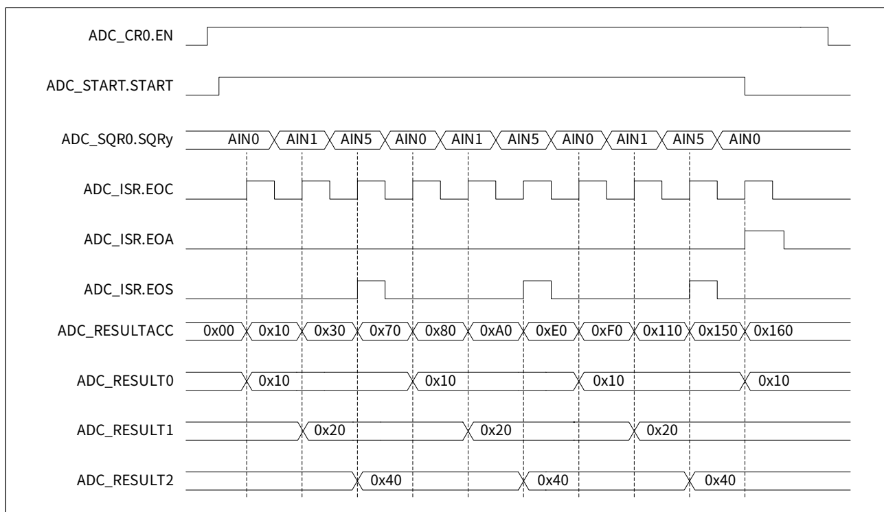
Figure 23-10 Accumulation conversion timing diagram
