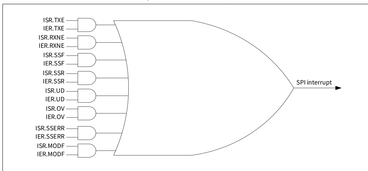
Figure 20-11 SPI interrupts
