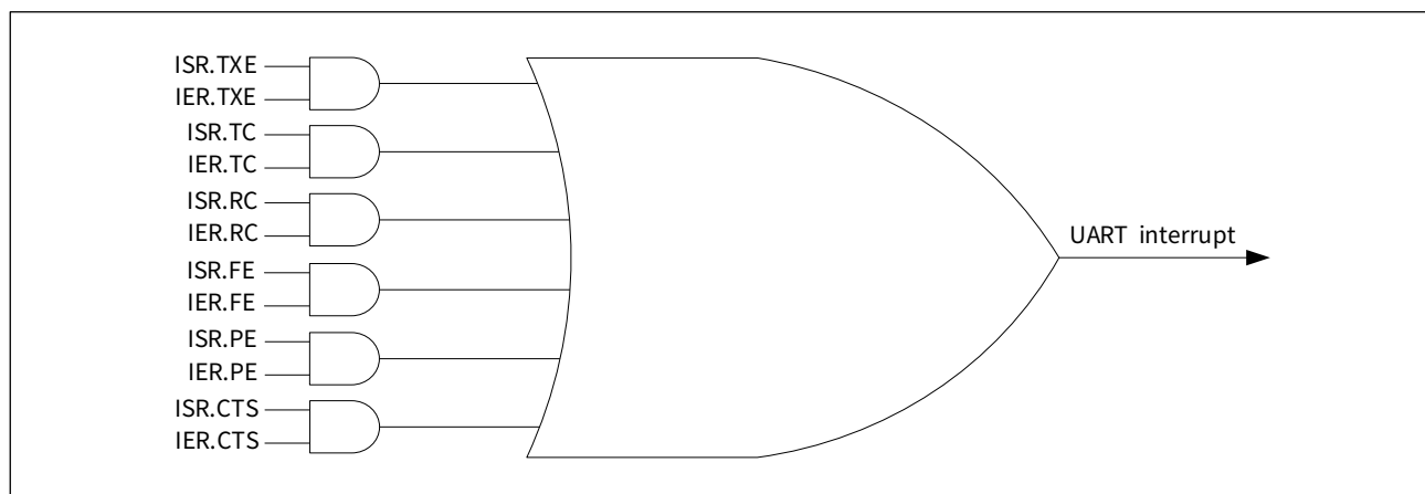
Figure 19-9 Schematic diagram of UART interrupt structure
