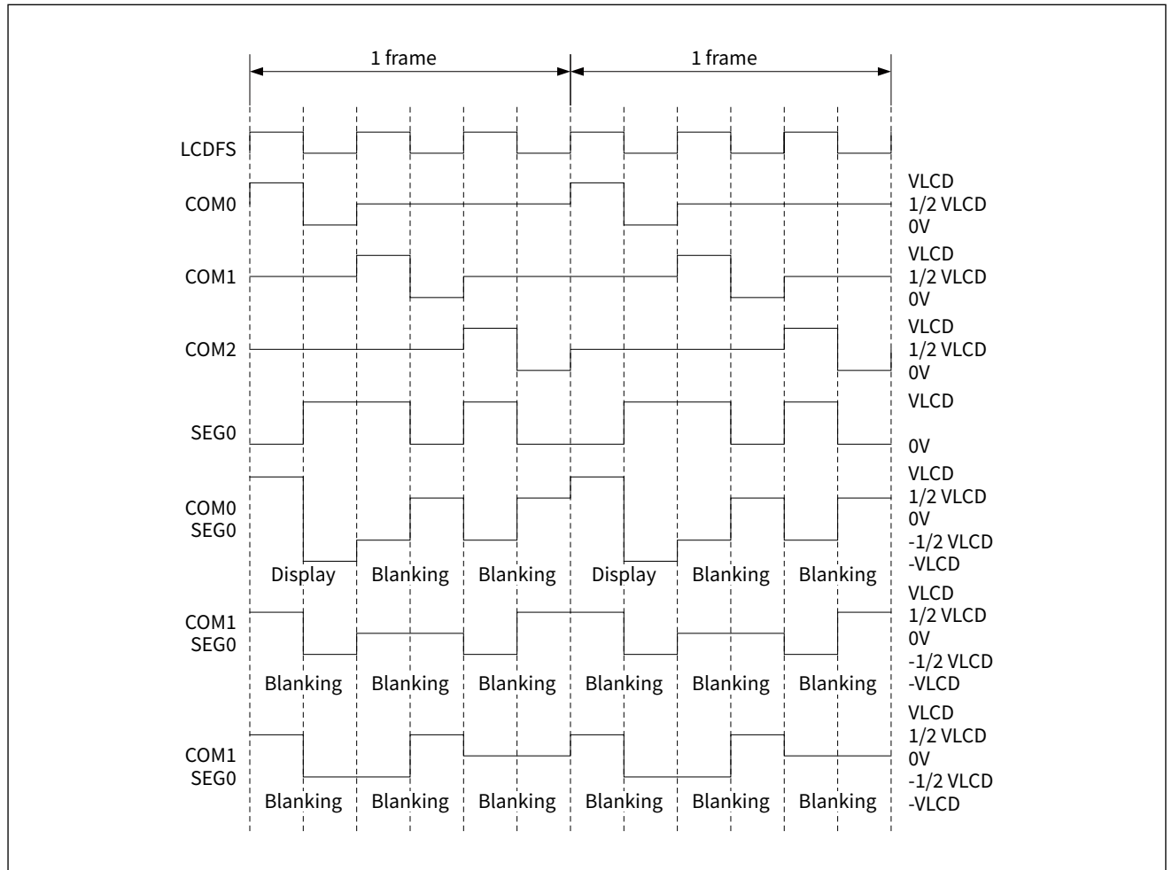
Figure 27-6 1/3 Duty 1/2 Bias driving waveform
