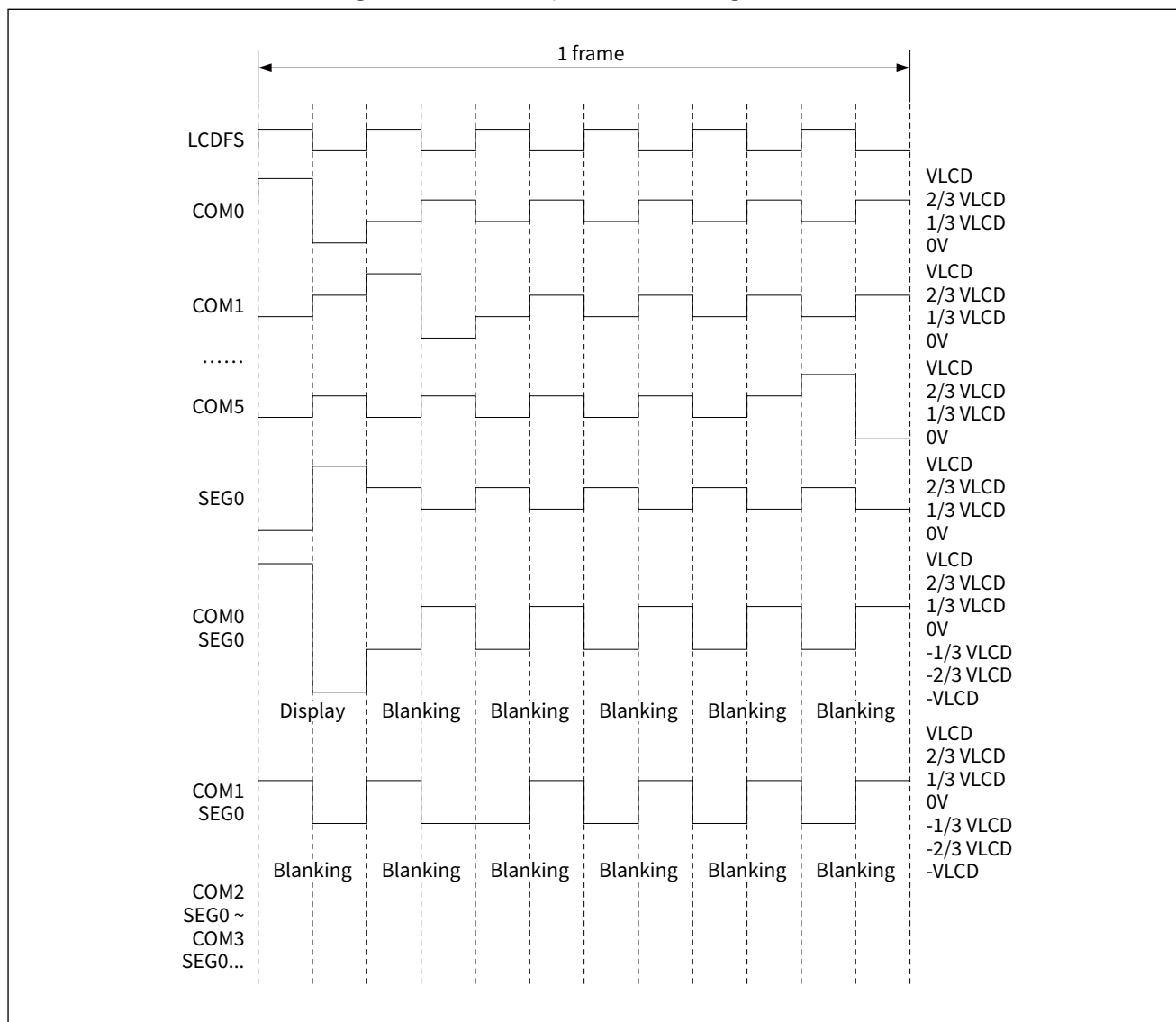
Figure 27-8 1/6 Duty 1/3 Bias driving waveform
