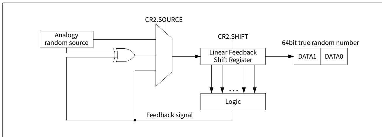
Figure 26-1 TRNG functional block diagram
