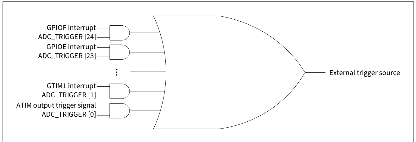
Figure 23-11 Schematic diagram of external trigger source for ADC conversion
