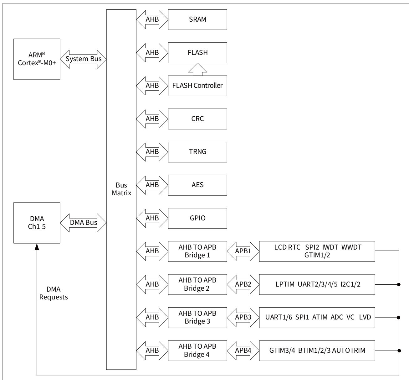
Figure 2-1 System architecture
