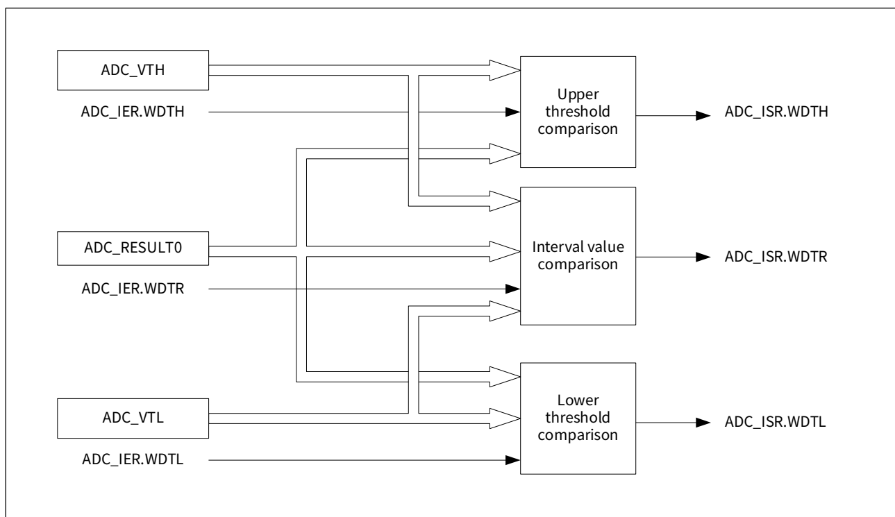
Figure 23-12 Schematic diagram of ADC threshold comparison
