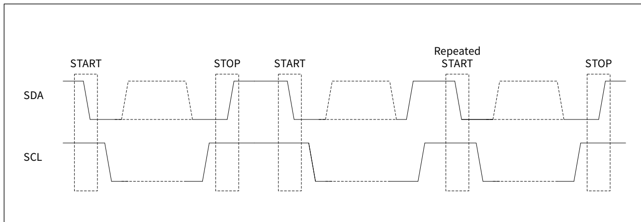
Figure 21-2 Start and stop signals
