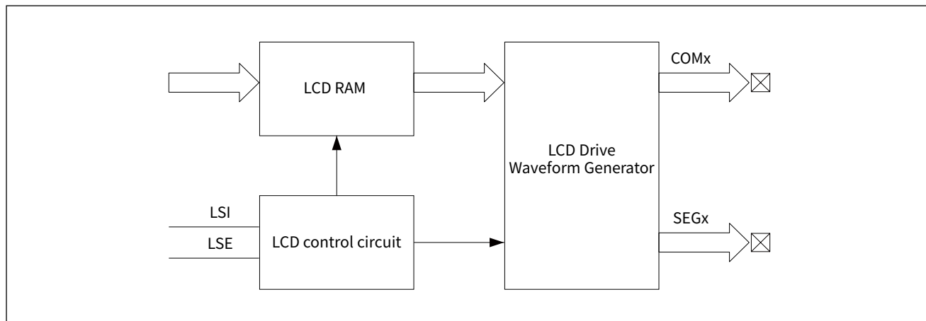
Figure 27-1 LCD functional block diagram
