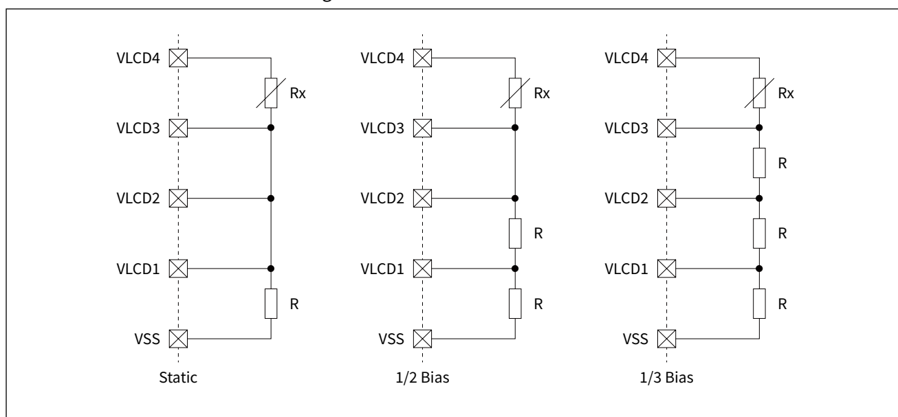
Figure 27-2 External Resistor Mode
