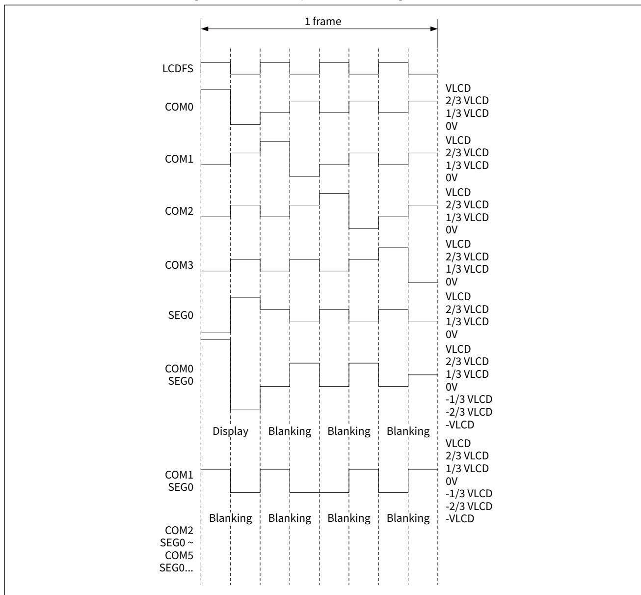
Figure 27-7 1/4 Duty 1/3 Bias driving waveform
