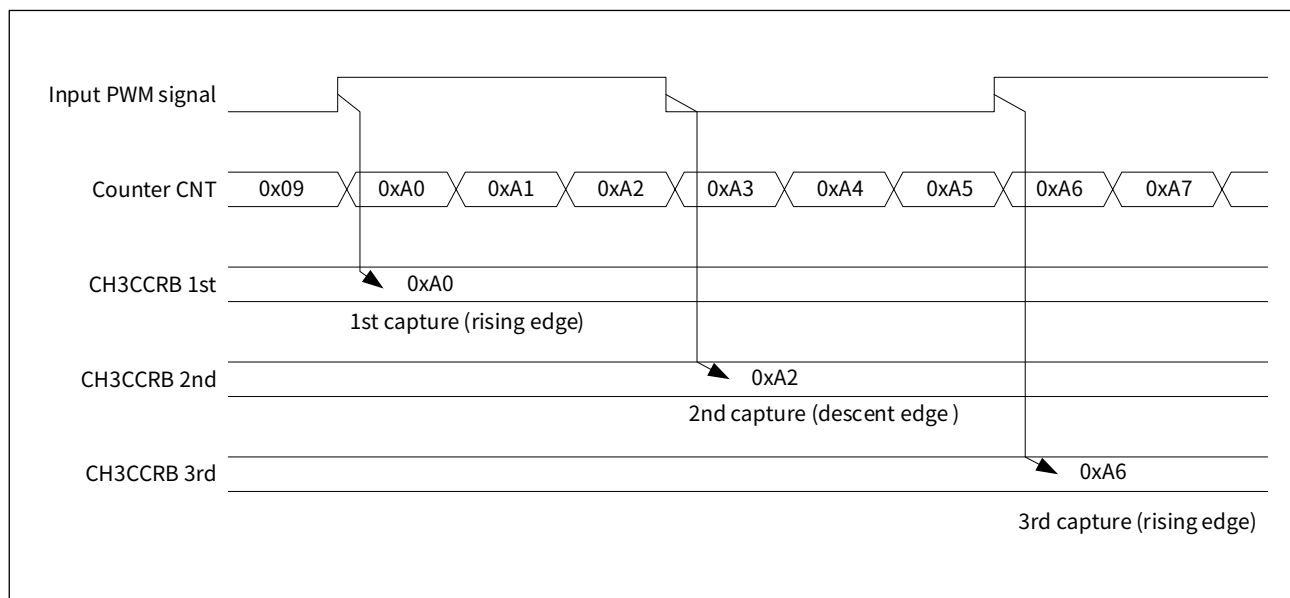
Figure 16-20 Schematic diagram of PWM measurement
