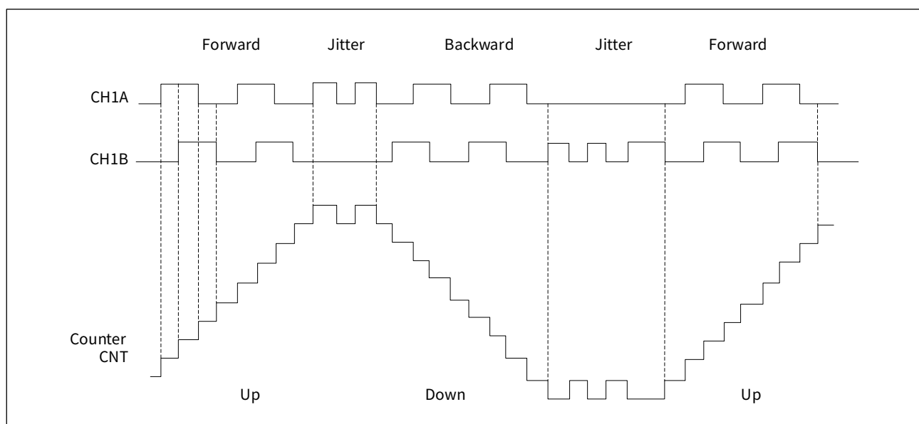
Figure 16-33 Encoding counting operation example
