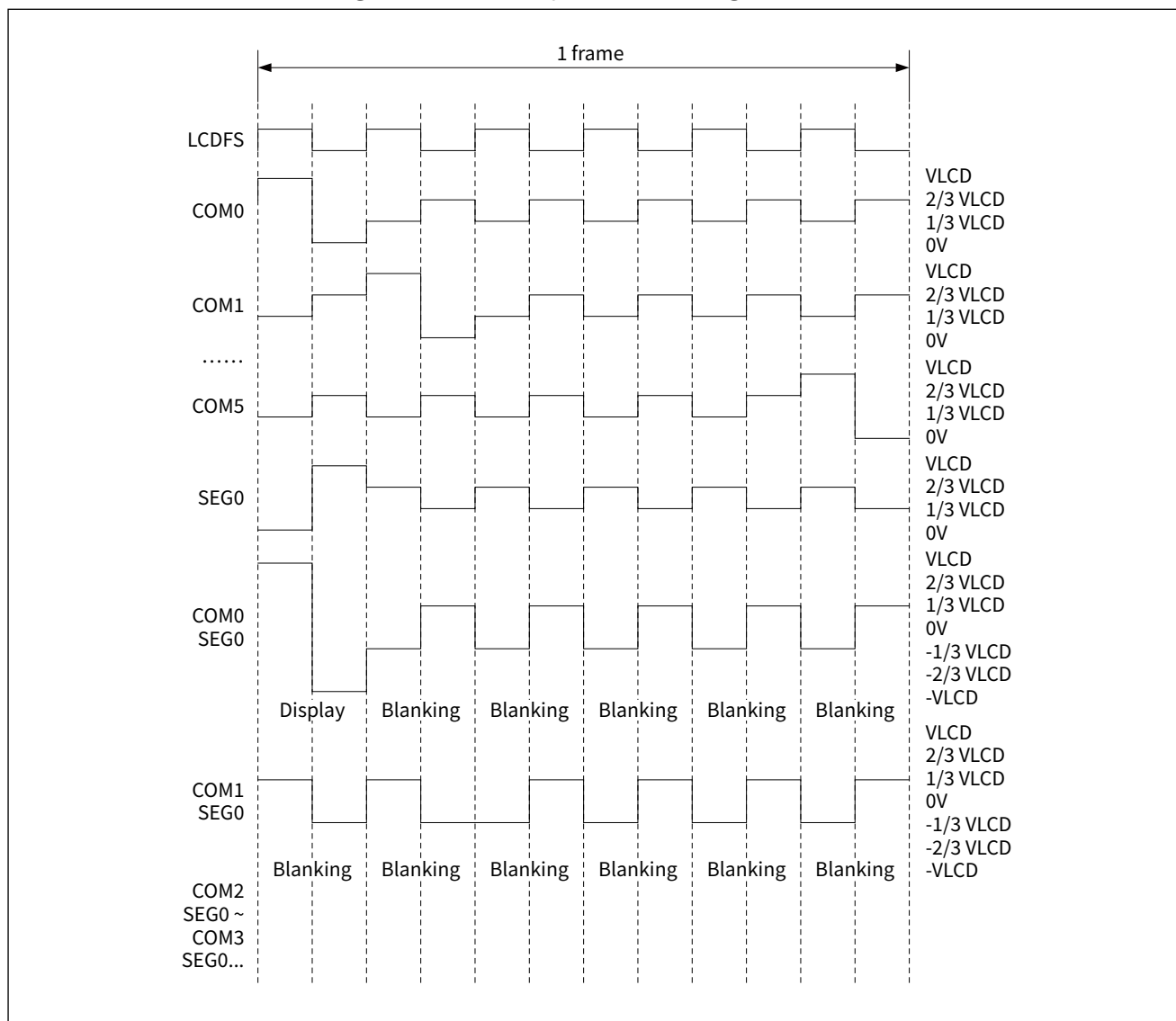
Figure 26-8 1/6 Duty 1/3 Bias driving waveform
