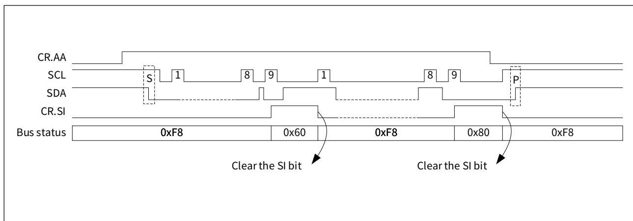
Figure 21-11 The status synchronization diagram of slave receive mode
