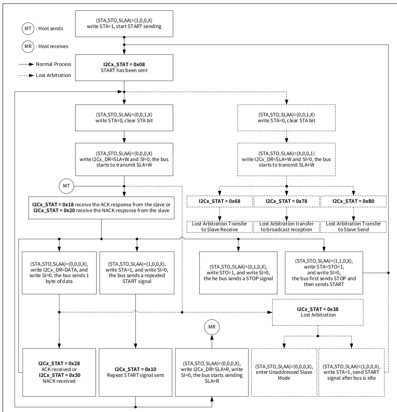
Figure 21-8 Master transmit mode flow and register status
