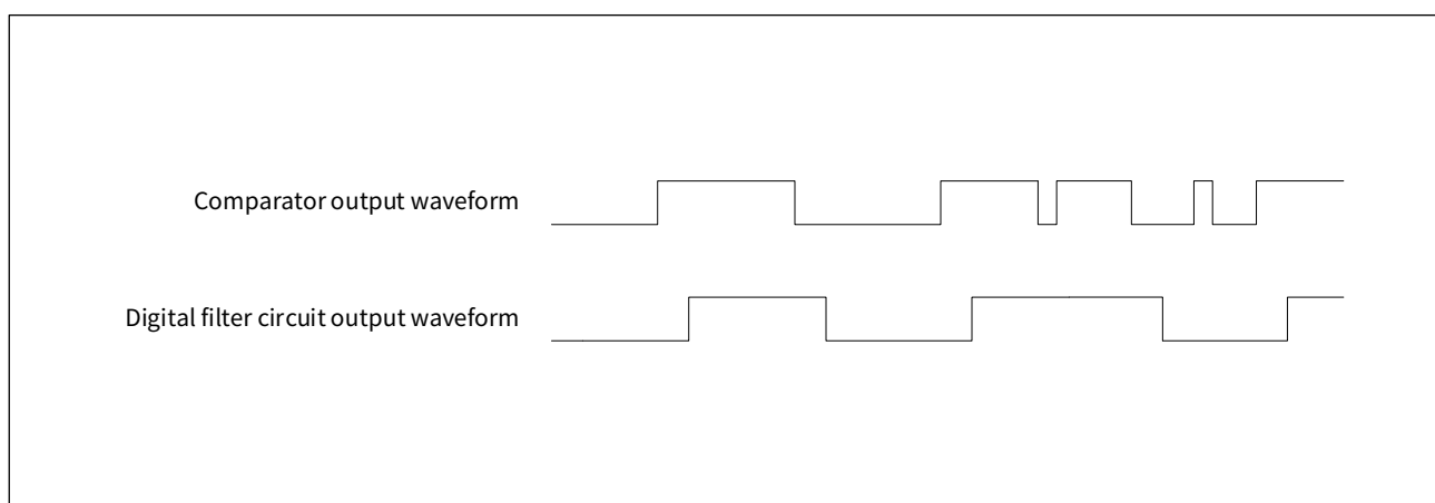
Figure 24-2 VC filter response time
