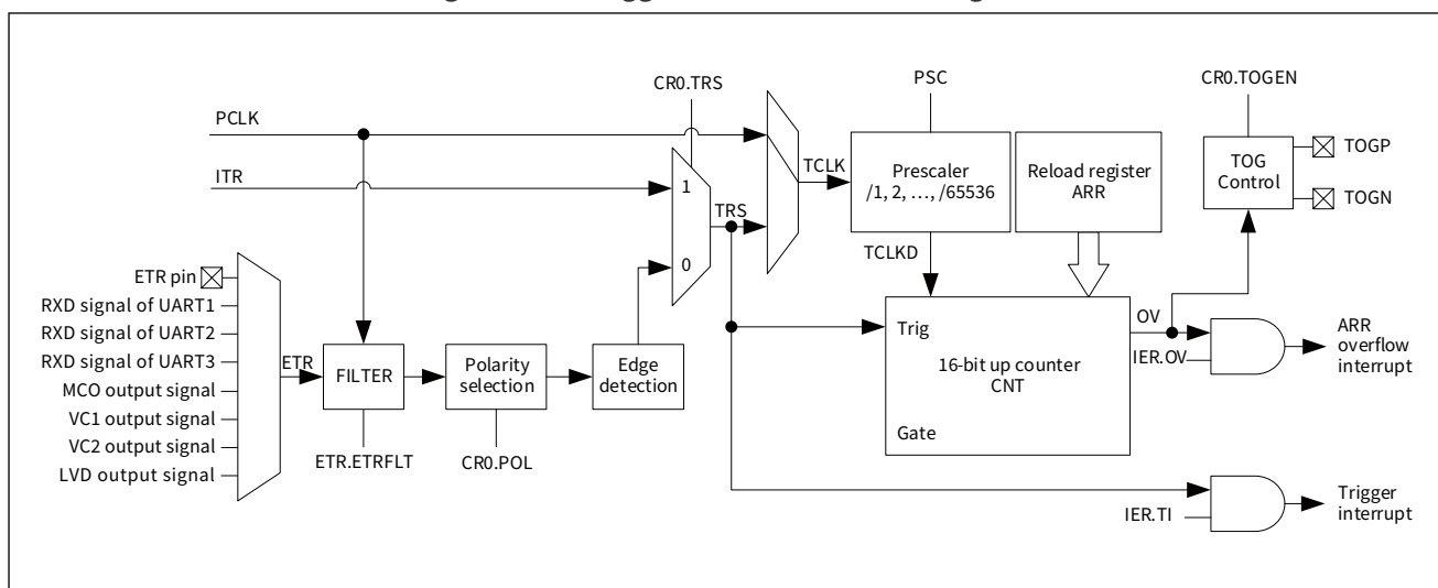
Figure 15-9 Trigger start mode block diagram
