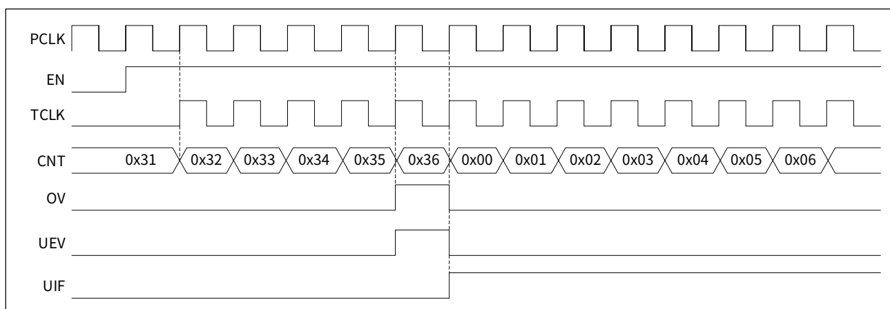
Figure 16-2 Upcounting, internal clock divided by 1
