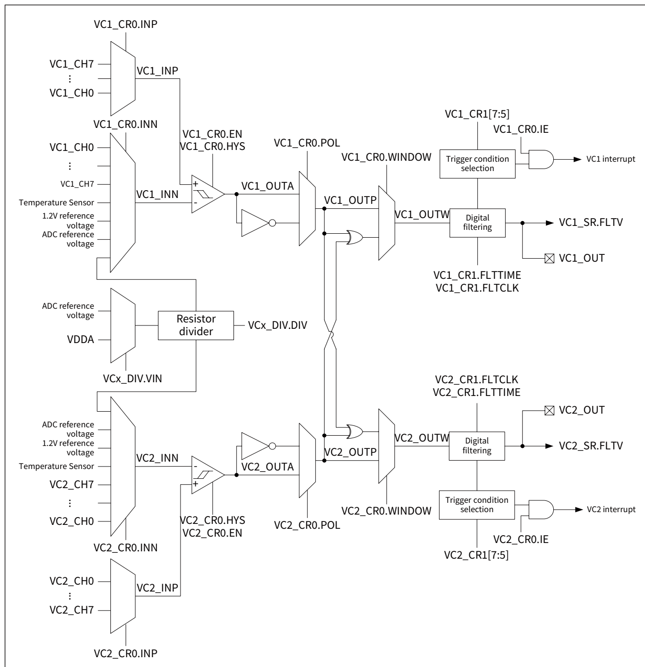
Figure 24-1 VC functional block diagram
