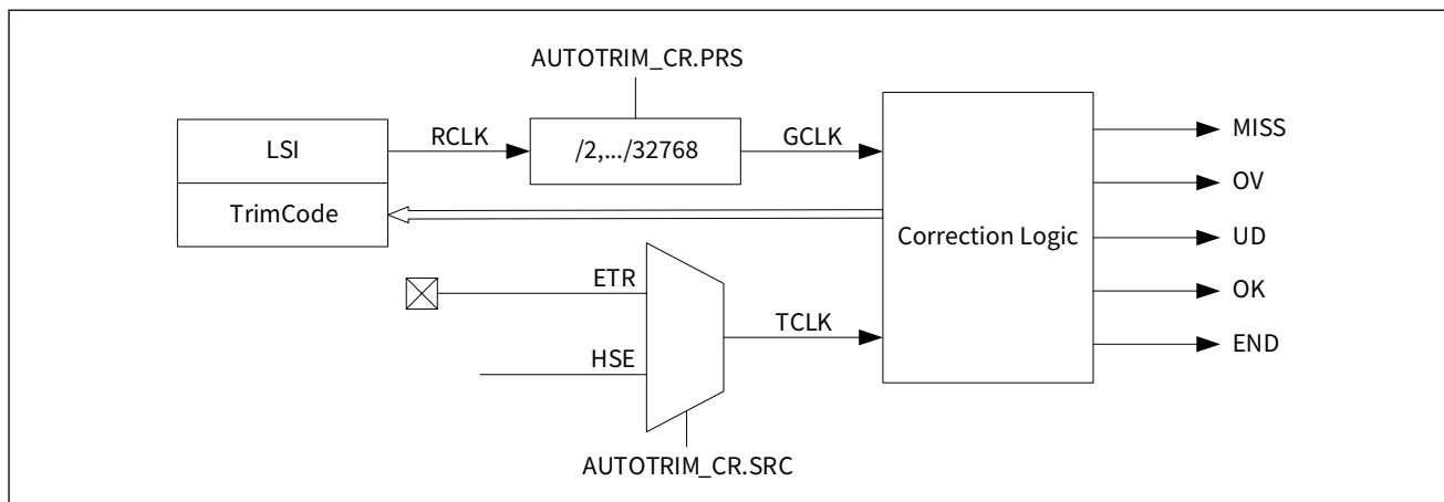
Figure 11-4 LSI Calibration Mode Functional Block Diagram
