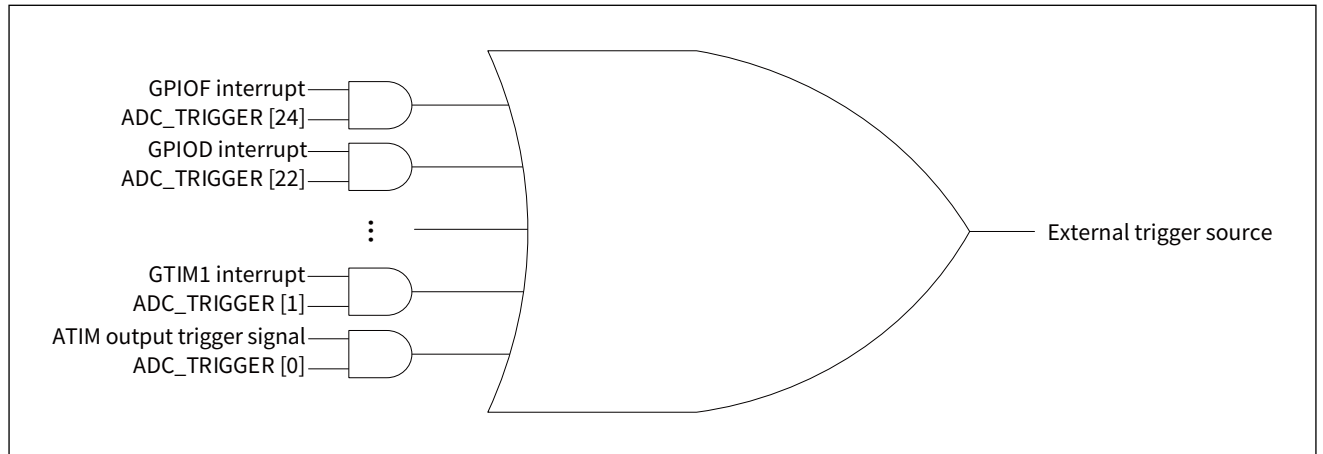
Figure 23-12 Schematic diagram of external trigger source for ADC conversion
