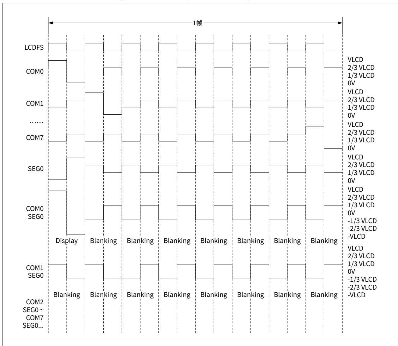
Figure 26-9 1/8 Duty 1/3 Bias driving waveform
