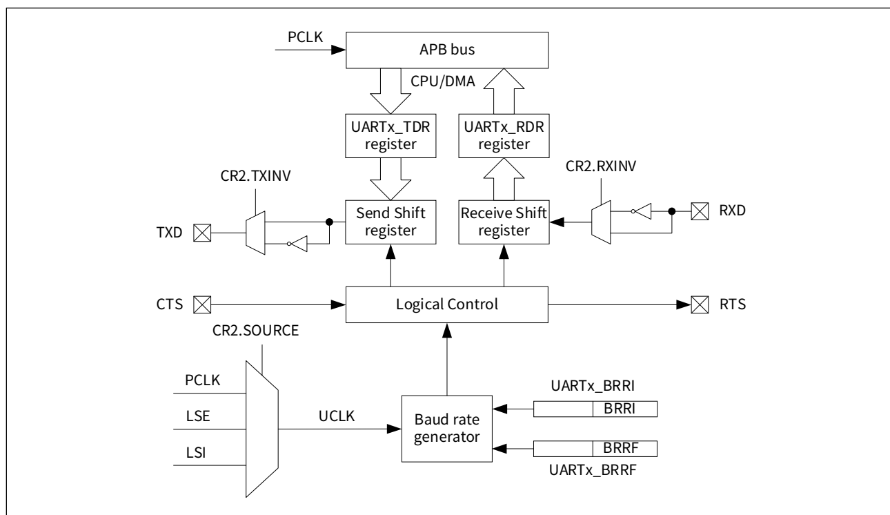
Figure 19-1 UART functional block diagram
