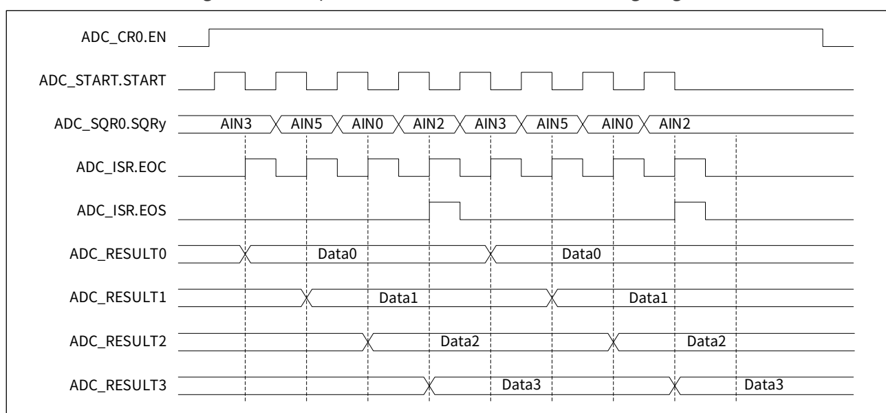
Figure 23-9 Sequence intermittent conversion timing diagram
