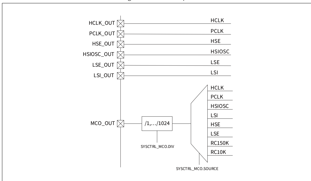
Figure 4-5 Clock output
