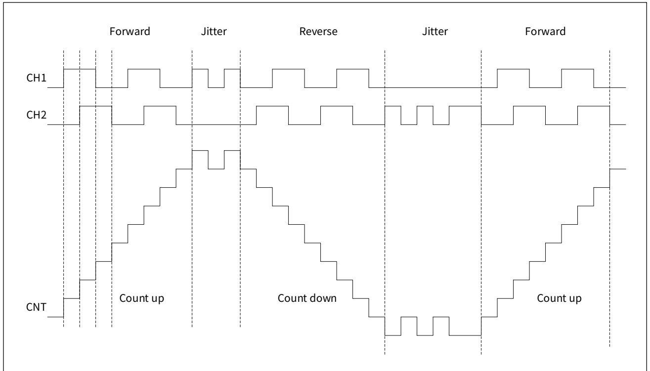
Figure 14-7 Encoder mode count example
