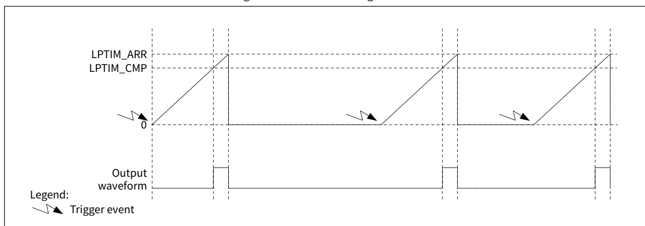
Figure 14-3 LPTIM Single Mode
