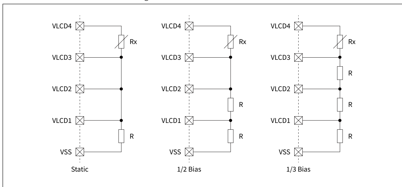
Figure 26-2 External Resistor Mode
