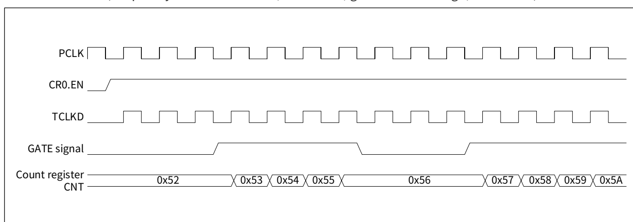
Figure 15-12 Timing diagram of gated mode (frequency division ratio is 1, PSC=0x00, gated is active high, POL=0x00)
