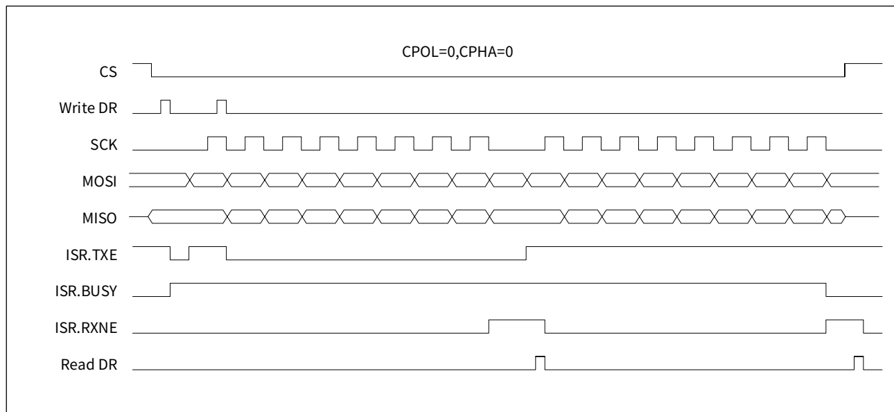
Figure 20-5 Master transmit and receive timing in full-duplex mode (two bytes)
