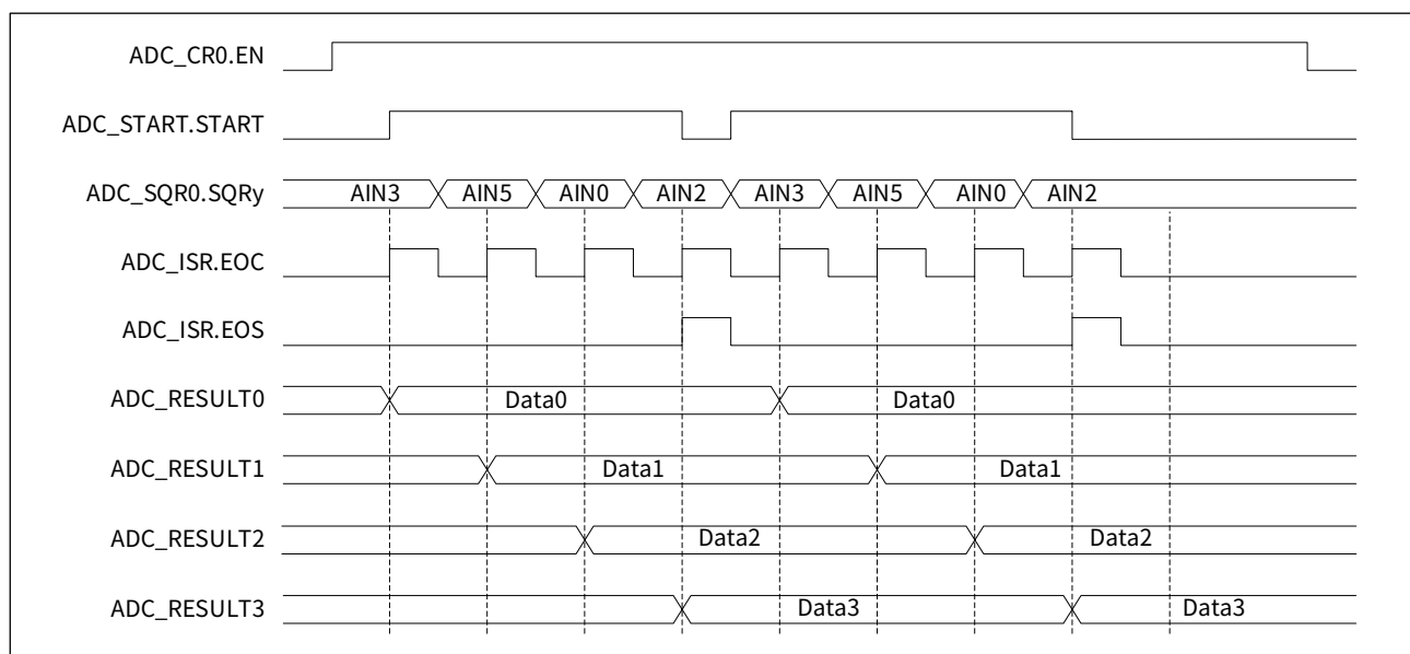
Figure 23-7 Sequence scan conversion timing diagram
