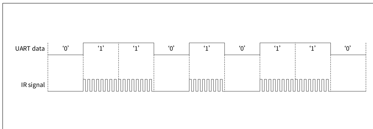
Figure 22-4 UART modulation mode
