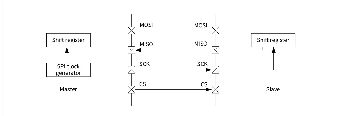
Figure 20-9 Master single receiving, slave single transmitting mode
