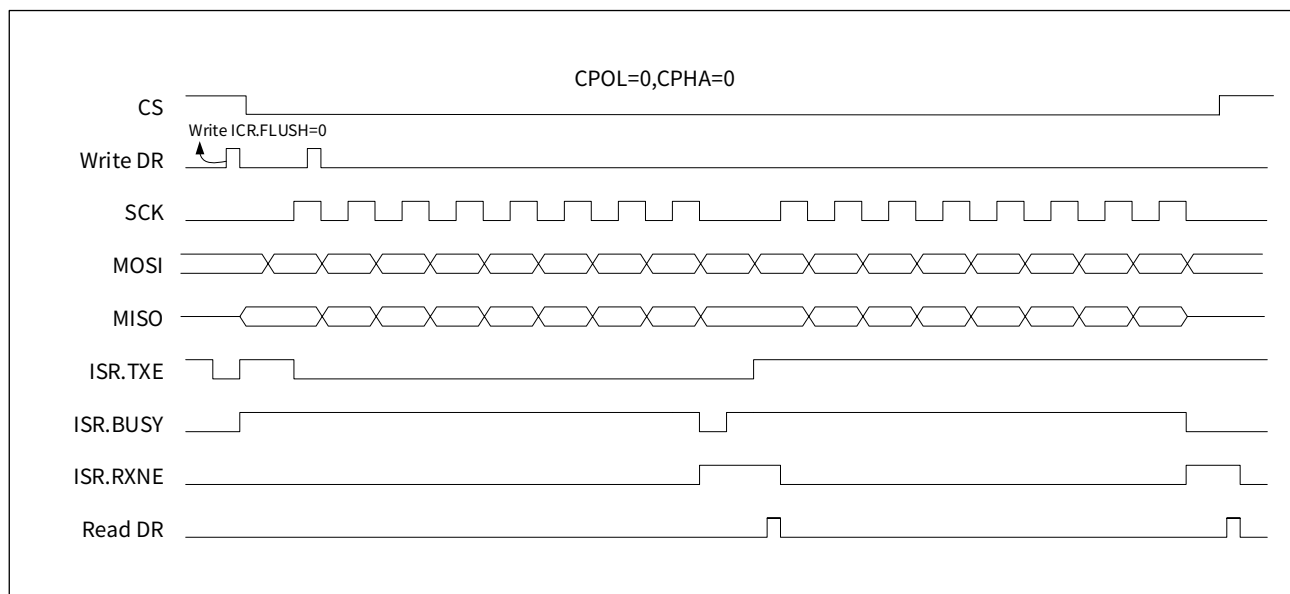
Figure 20-6 Slave transmit and receive timing in full-duplex mode (two bytes)
