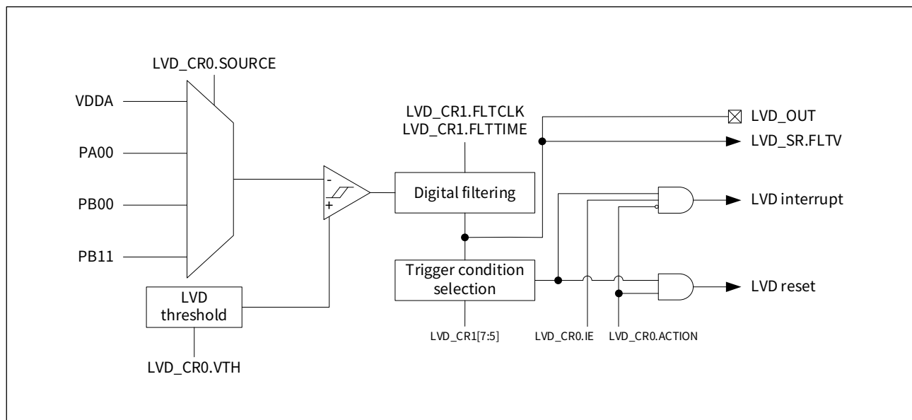
Figure 25-1 LVD functional block diagram
