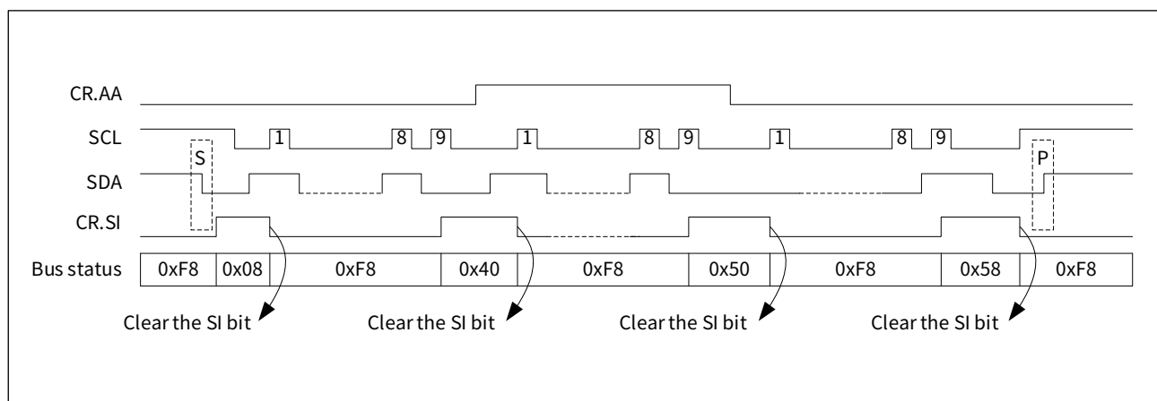
Figure 21-9 The status synchronization diagram of master receive mode
