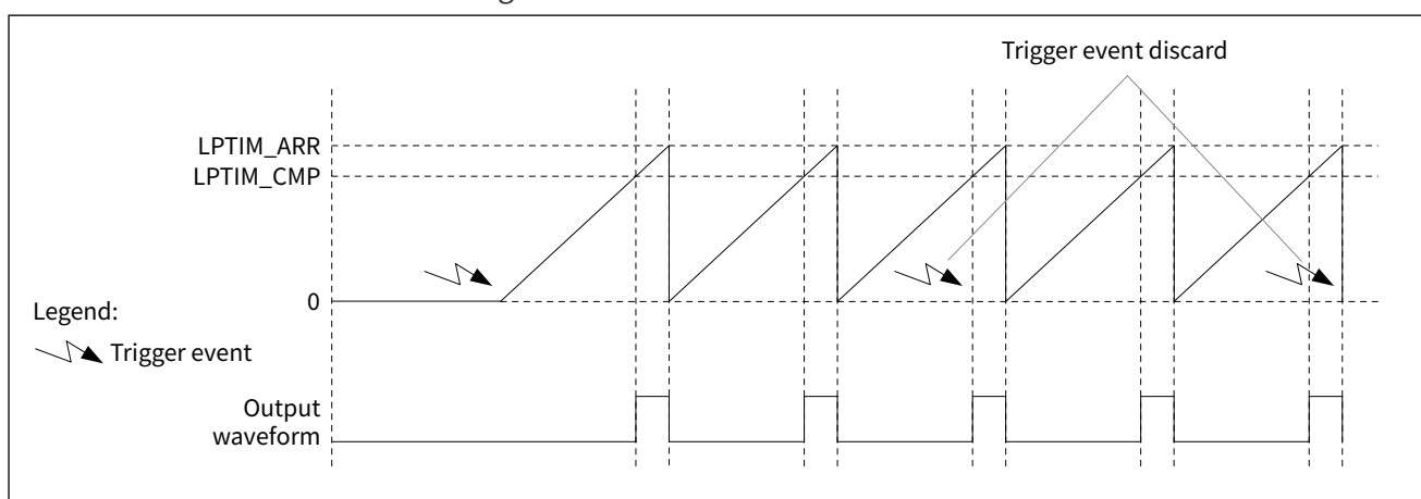
Figure 14-5 LPTIM Continuous Mode
