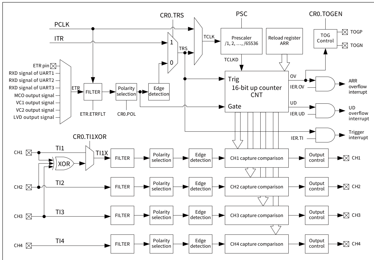
Figure 15-1 GTIM functional block diagram
