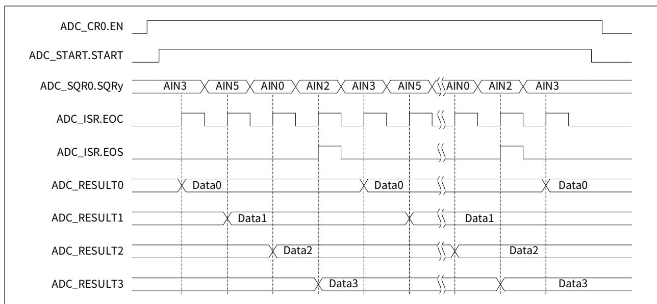
Figure 23-6 Sequence continuous conversion timing diagram
