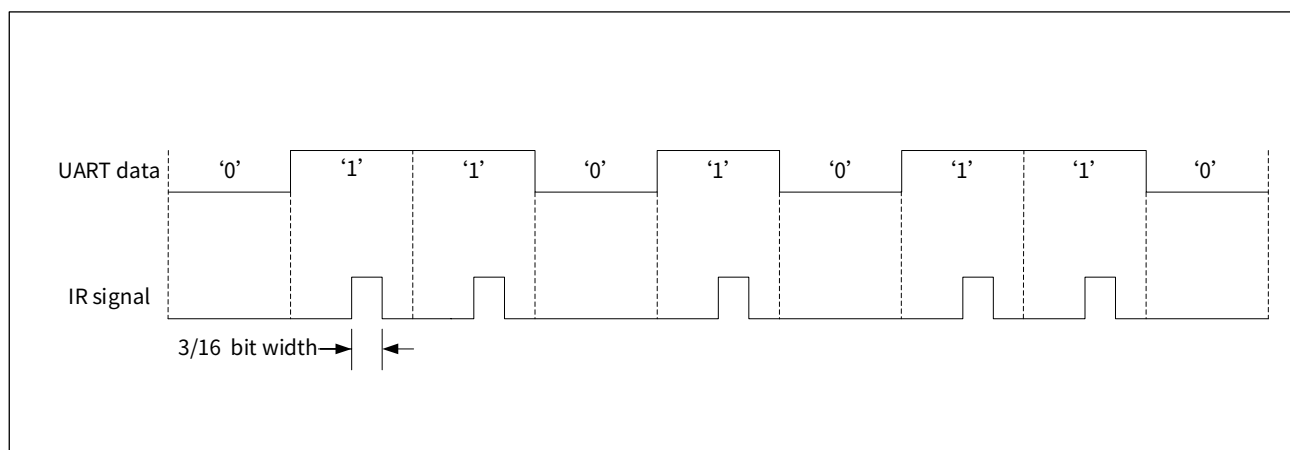
Figure 22-5 High-speed UART modulation mode
