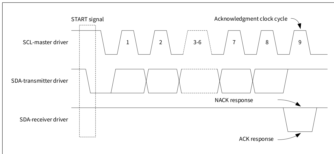
Figure 21-4 Transmission response
