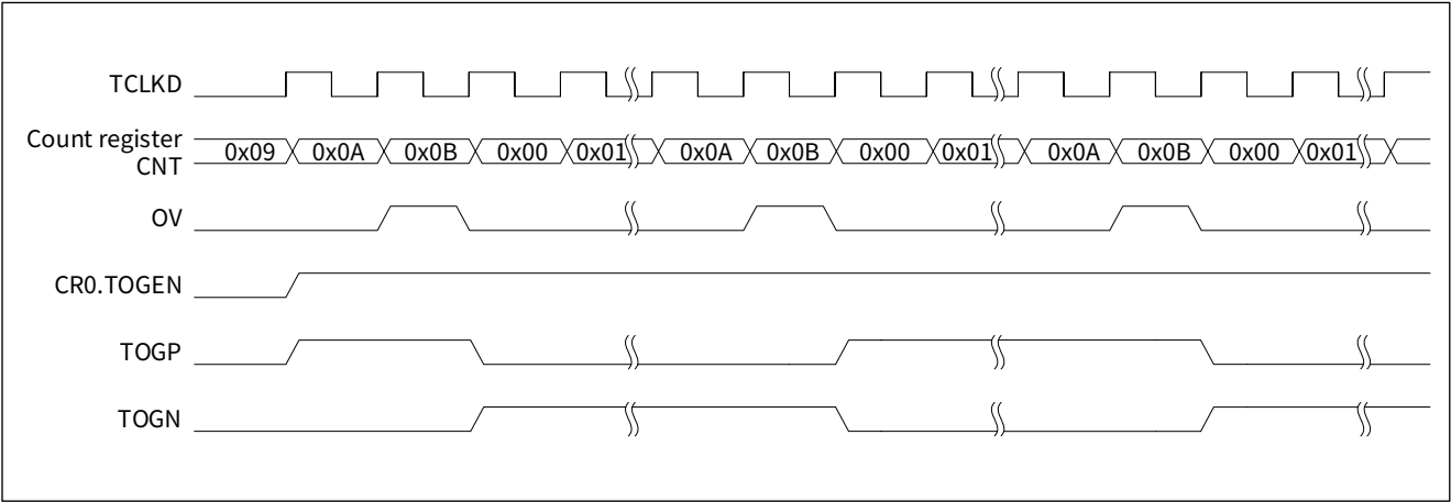
Figure 15-5 Schematic diagram of level flip output (continuous counting mode, ARR=0x0B)
