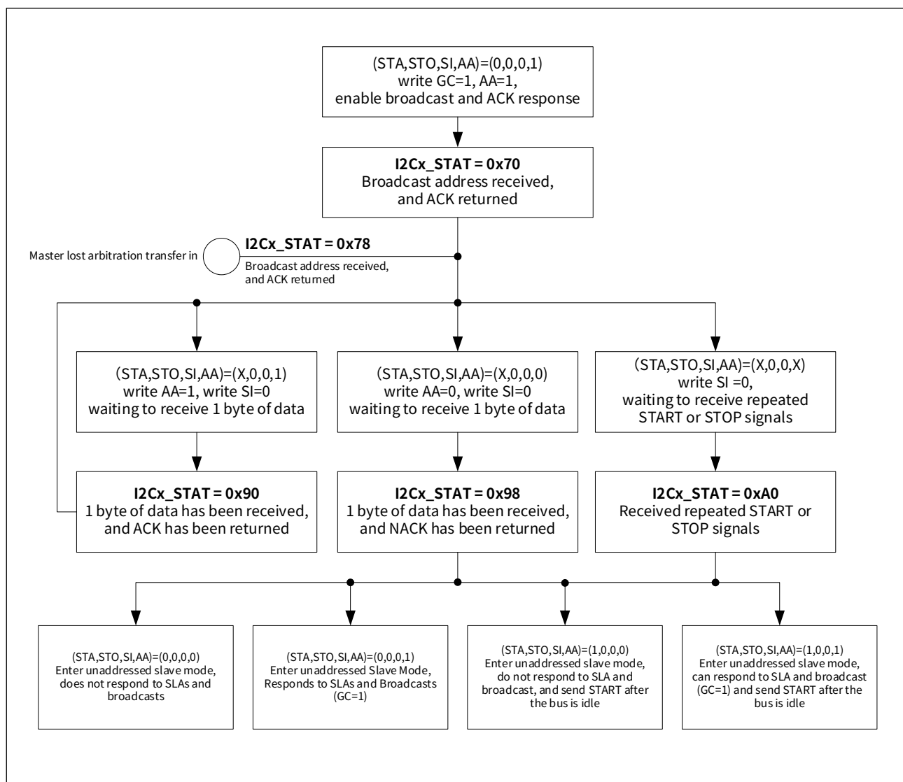
Figure 21-15 Broadcast receive mode flow and register status
