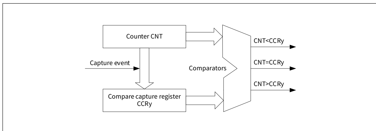
Figure 15-4 Schematic diagram of the capture compare channel
