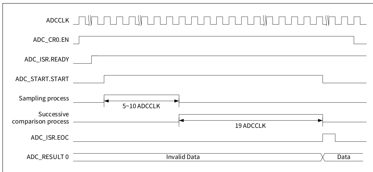
Figure 23-2 ADC conversion timing diagram
