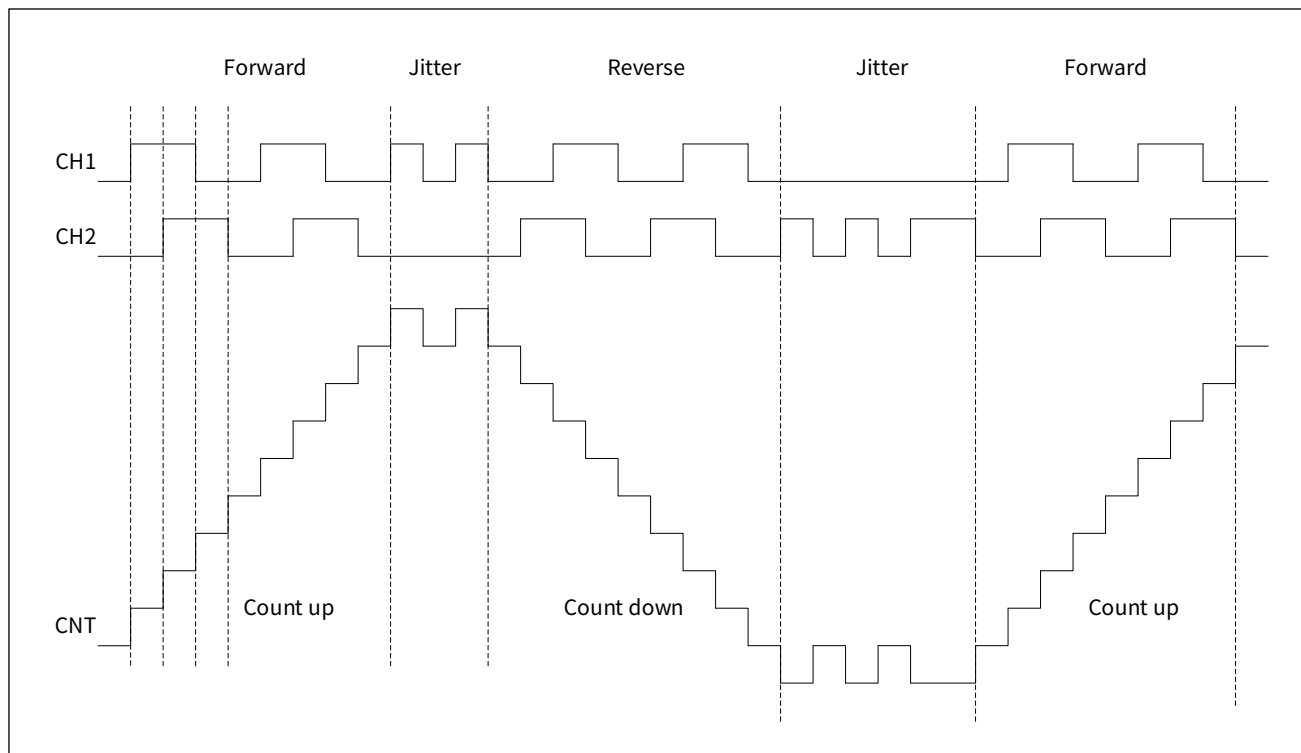
Figure 15-17 Example of counter operation in encoder mode
