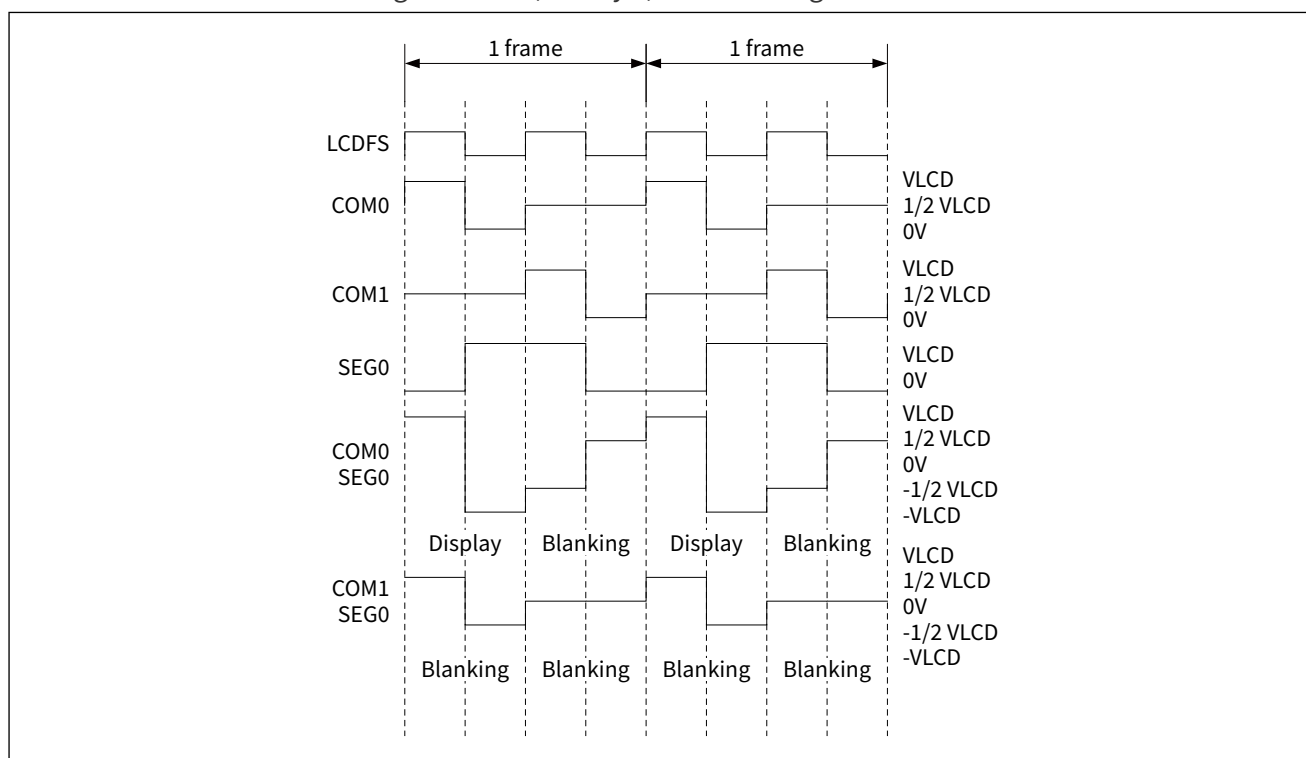
Figure 26-5 1/2 Duty 1/2 Bias driving waveform
