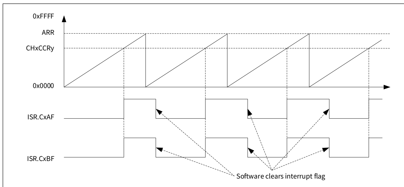
Figure 16-30 Edge-aligned mode compare match interrupt
