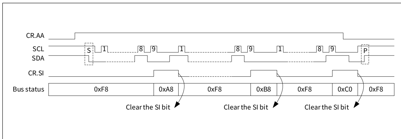
Figure 21-13 The status synchronization diagram of slave transmit mode
