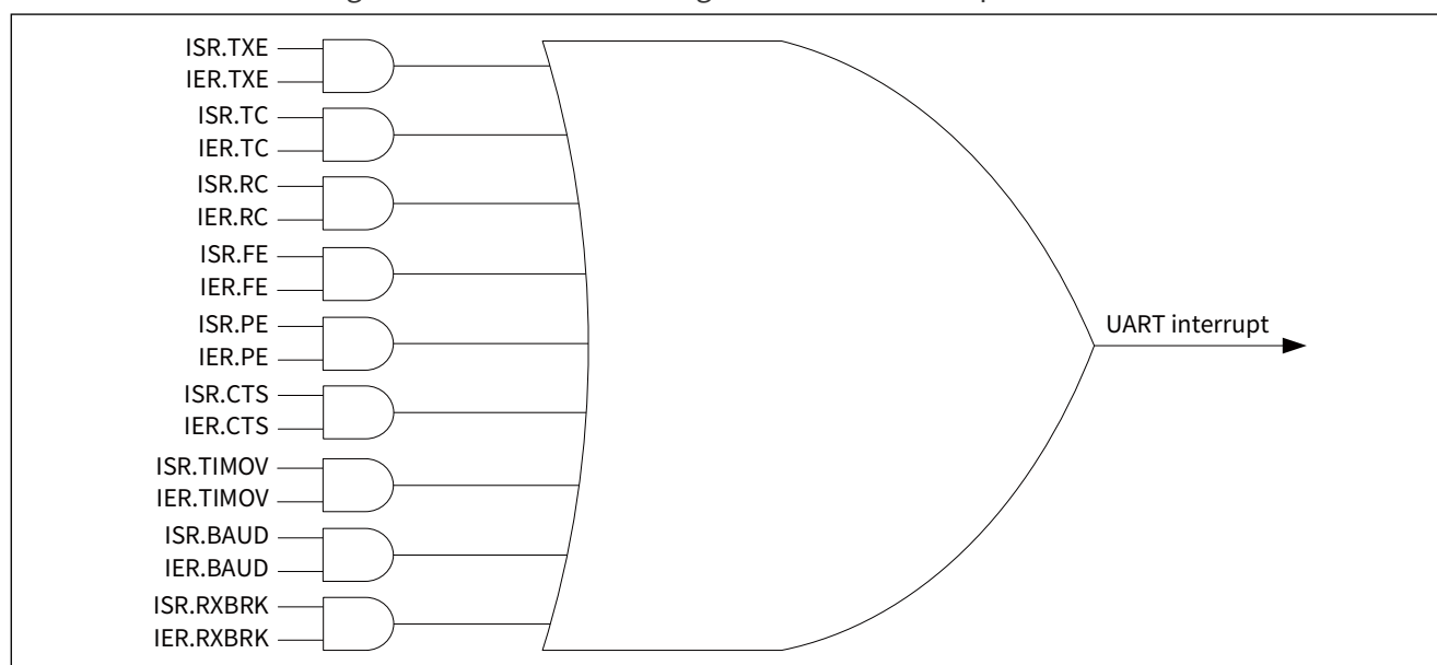
Figure 19-10 Schematic diagram of UART interrupt structure
