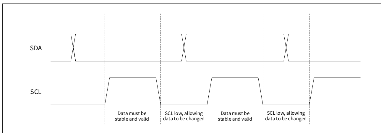
Figure 21-3 Data transmission
