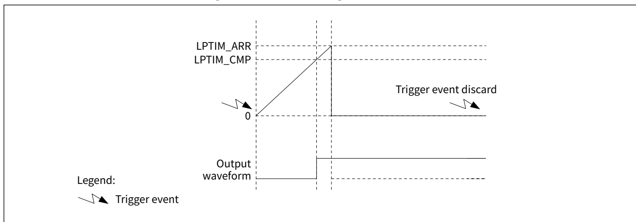
Figure 14-4 LPTIM Single Set Waveform
