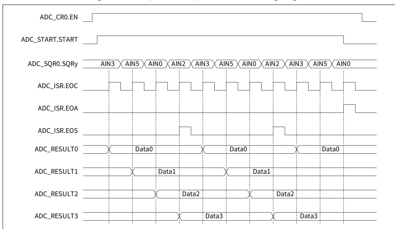
Figure 23-8 Sequence multiple conversion timing diagram
