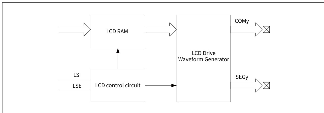
Figure 26-1 LCD functional block diagram
