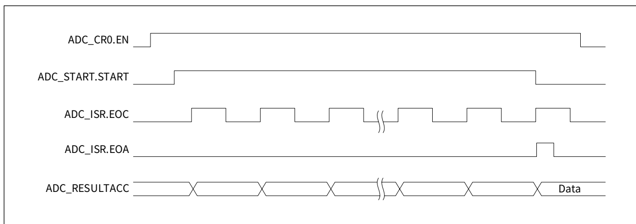
Figure 23-4 Single channel multiple conversion timing diagram
