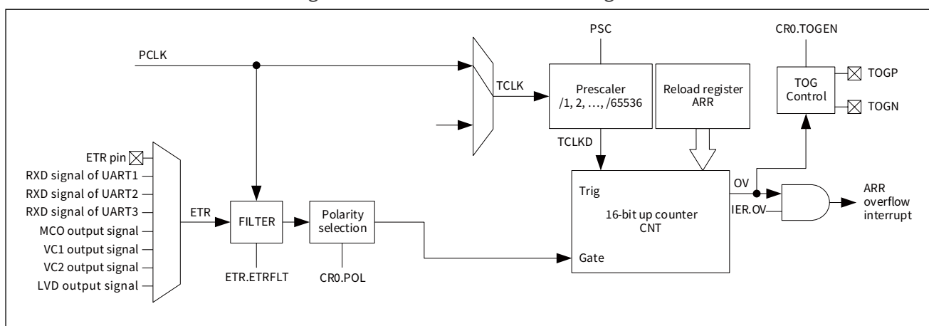
Figure 15-11 Gated mode block diagram
