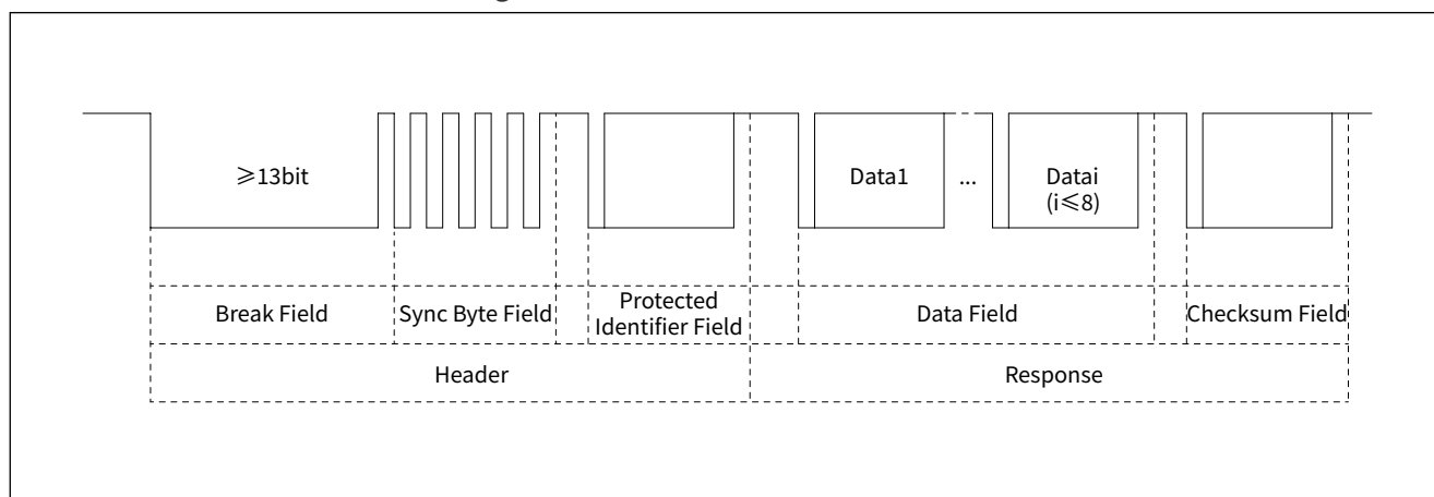
Figure 19-9 Structure of the LIN frame
