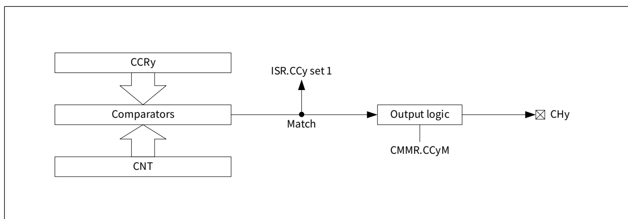
Figure 15-14 Output compare mode block diagram
