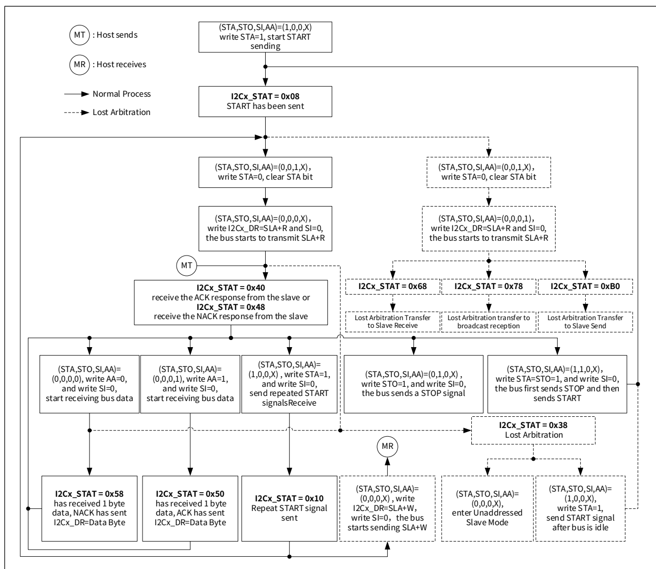
Figure 21-10 Master receive mode flow and register status
