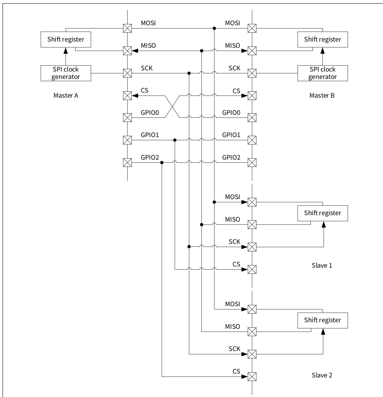
Figure 20-10 Multi-machine communication system
