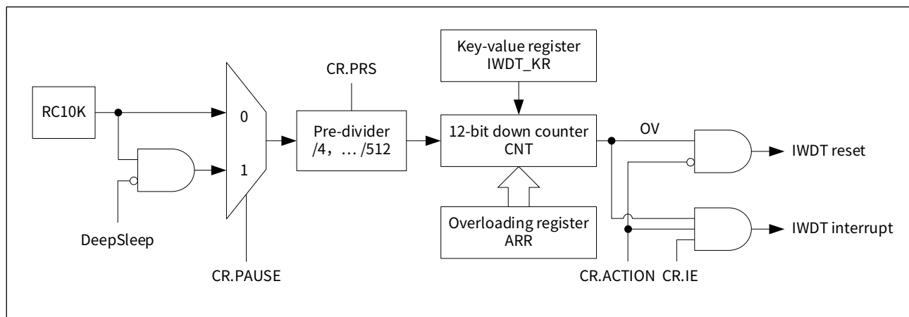
Figure 17-1 IWDT functional block diagram
