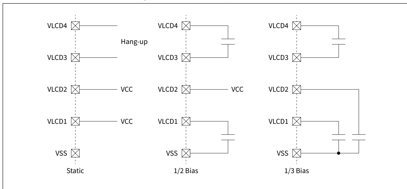
Figure 26-3 External Capacitor Mode
