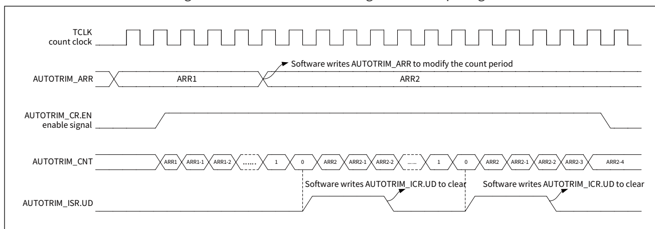
Figure 11-2 AUTOTRIM counting and interrupt flags
