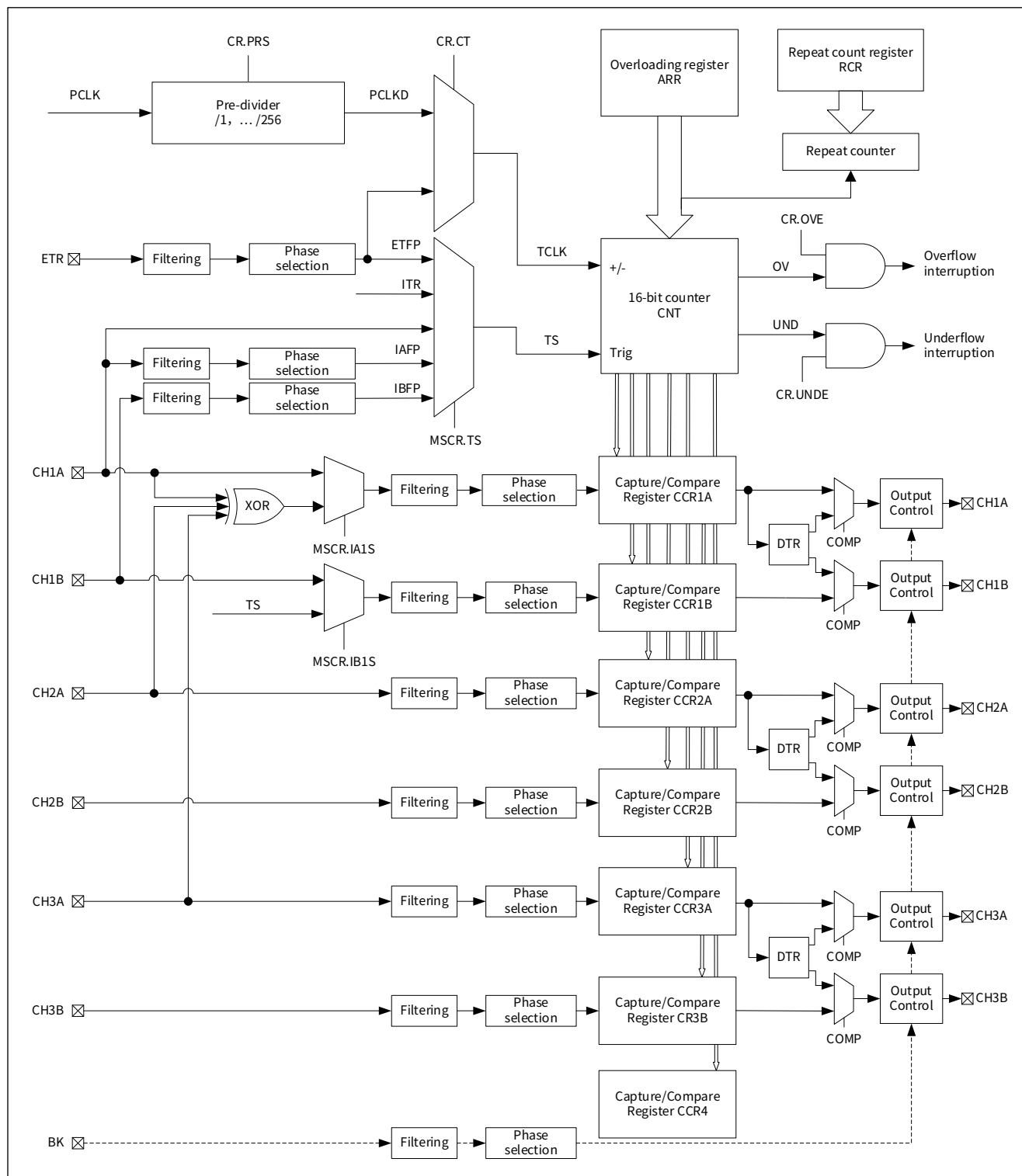
Figure 16-1 ATIM functional block diagram
