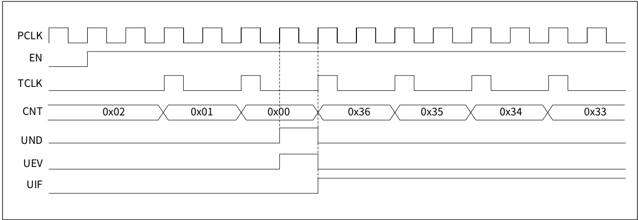
Figure 16-10 Downcounting, internal clock divided by 4
