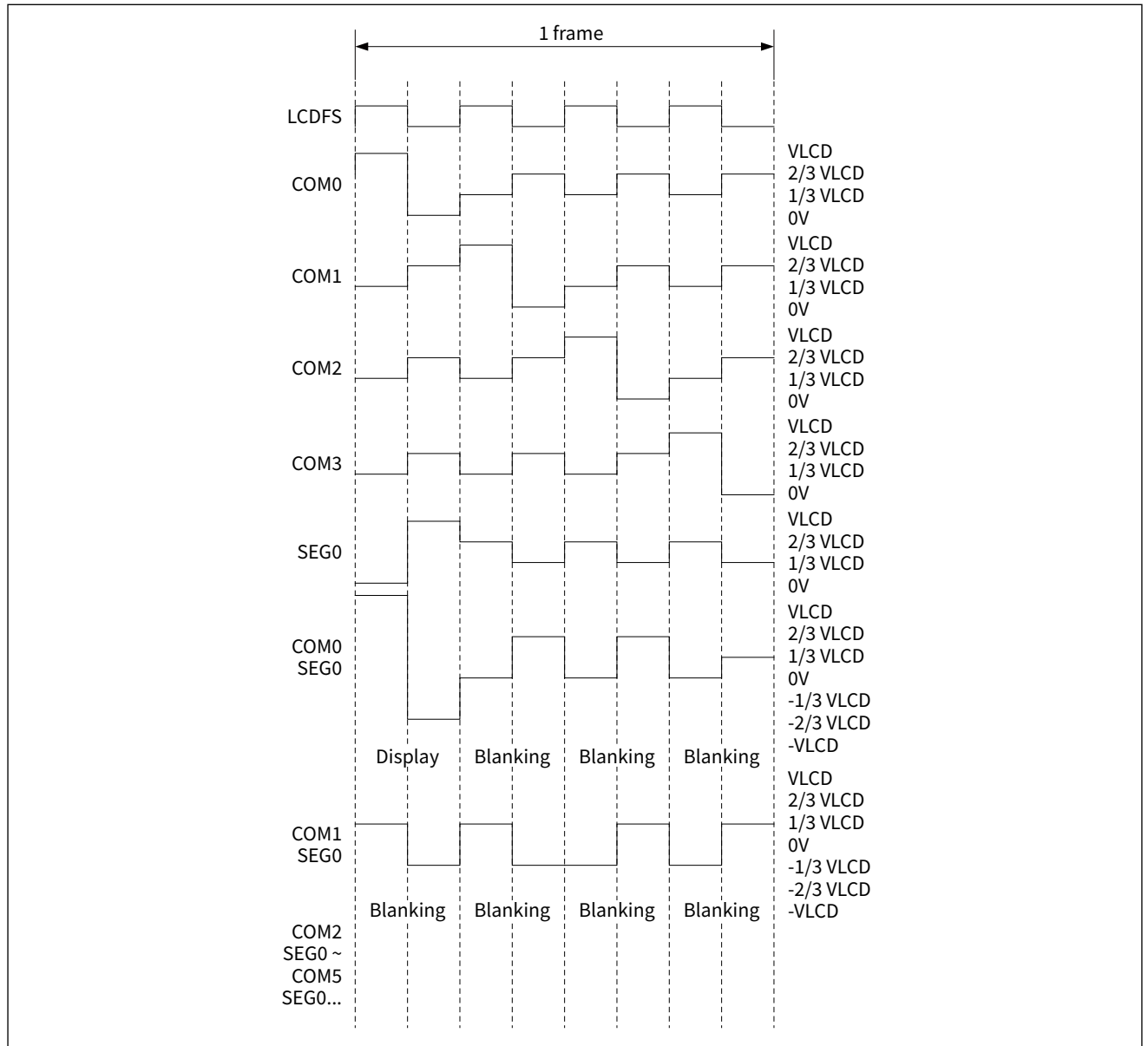
Figure 26-7 1/4 Duty 1/3 Bias driving waveform
