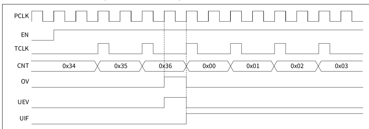
Figure 16-3 Upcounting, internal clock divided by 2
