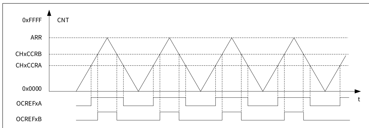
Figure 16-25 PWM mode 2, center Aligned, single-point comparison
