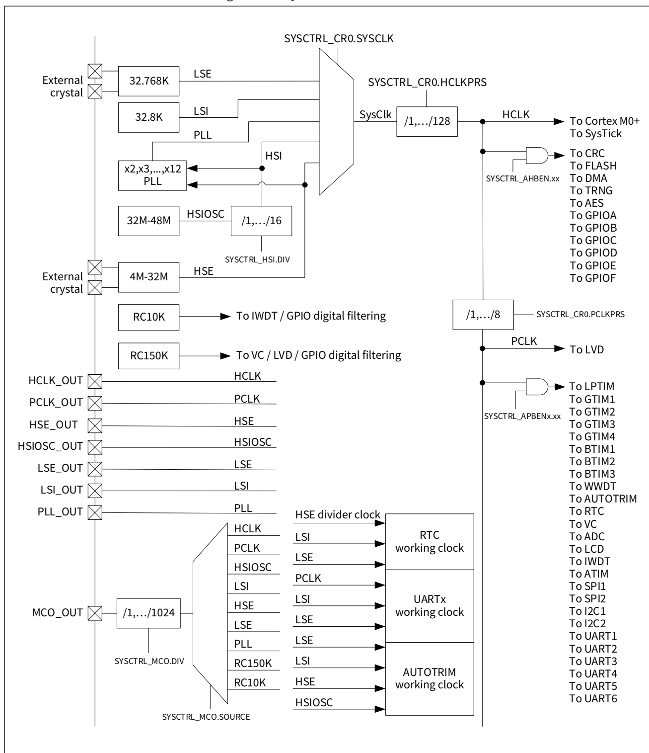
Figure 4-1 System internal clock tree
