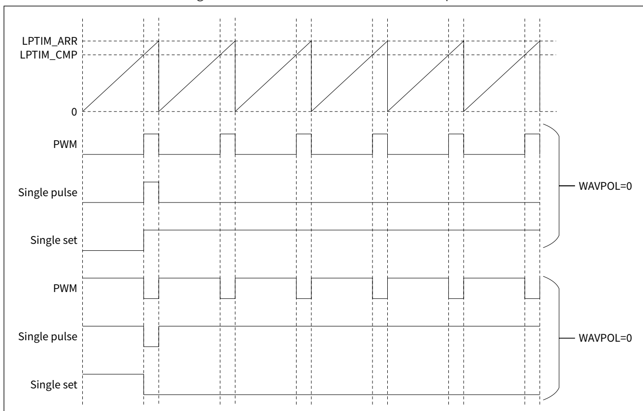
Figure 14-6 Three waveforms of LPTIM output
