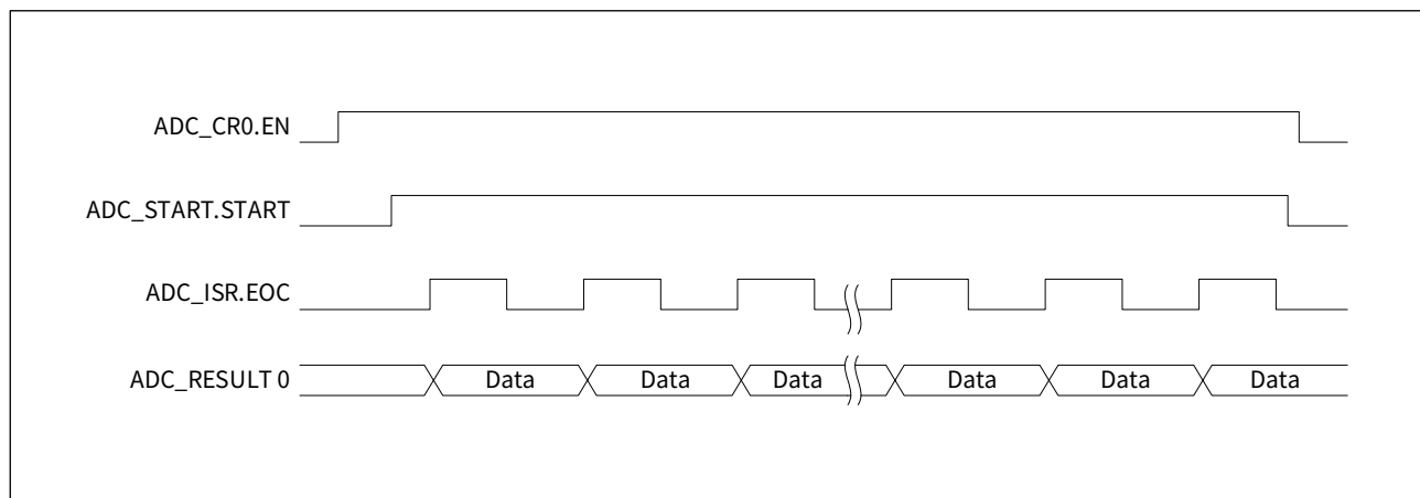
Figure 23-5 Single channel continuous conversion timing diagram
