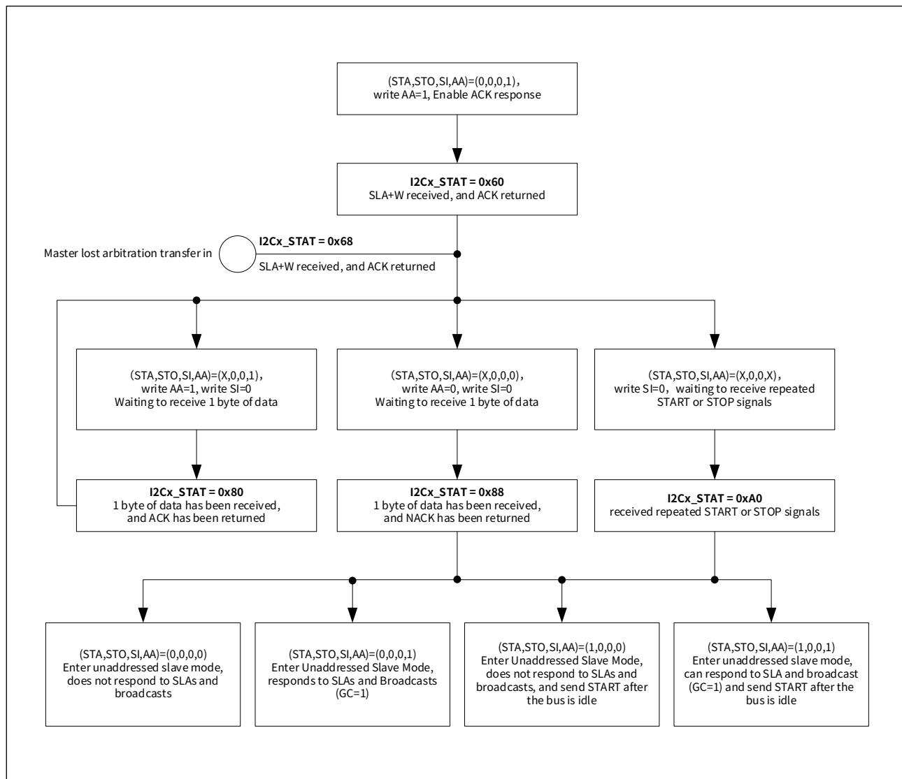
Figure 21-12 Slave receive mode flow and register status
