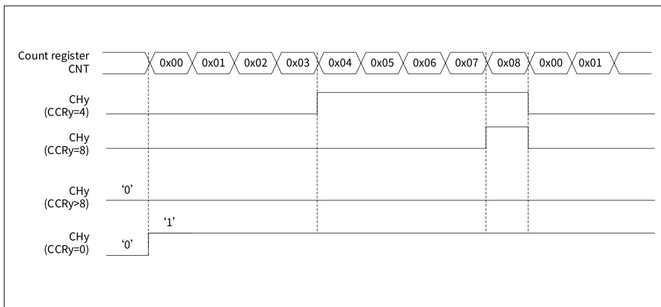
Figure 15-16 PWM waveform example
