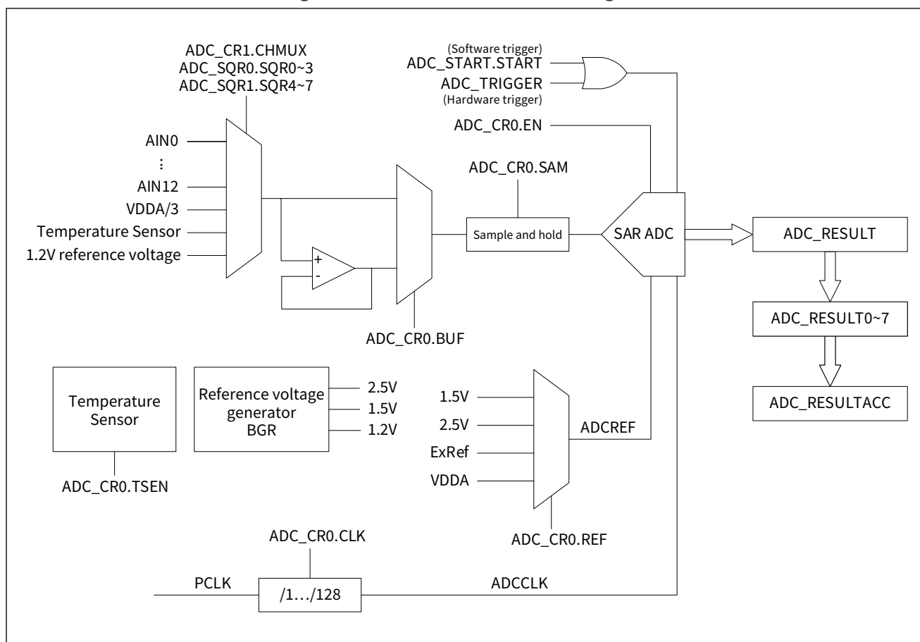
Figure 23-1 ADC functional block diagram
