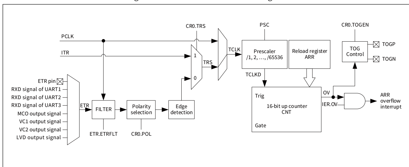
Figure 15-8 Counter mode block diagram
