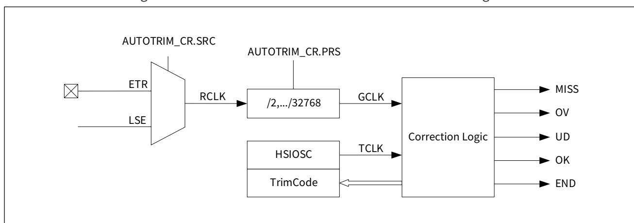
Figure 11-3 HSIOSC Calibration Mode Functional Block Diagram
