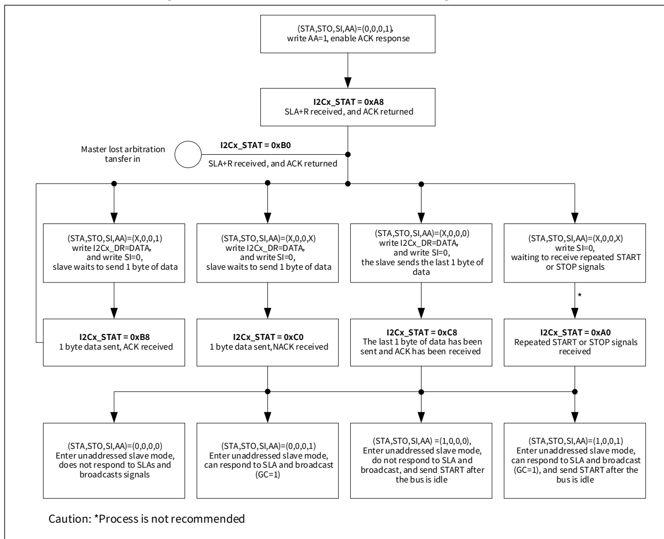
Figure 21-14 Slave transmit mode flow and register status
