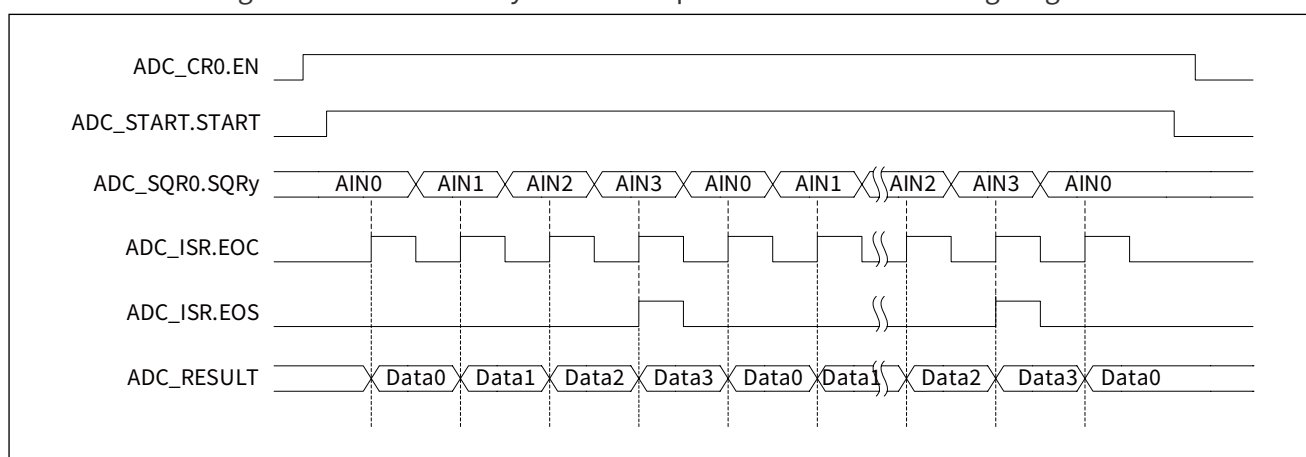
Figure 23-10 Channel-by-channel sequential conversion timing diagram
