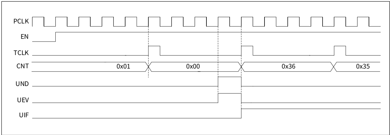
Figure 16-11 Downcounting, internal clock divided by N
