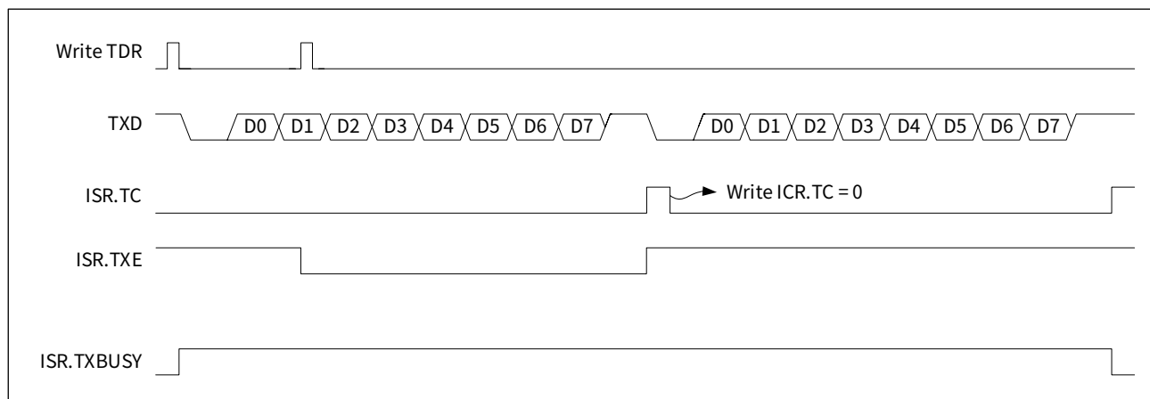
Figure 19-4 Transmit control sequence in asynchronous working mode (transmitting two bytes of data)
