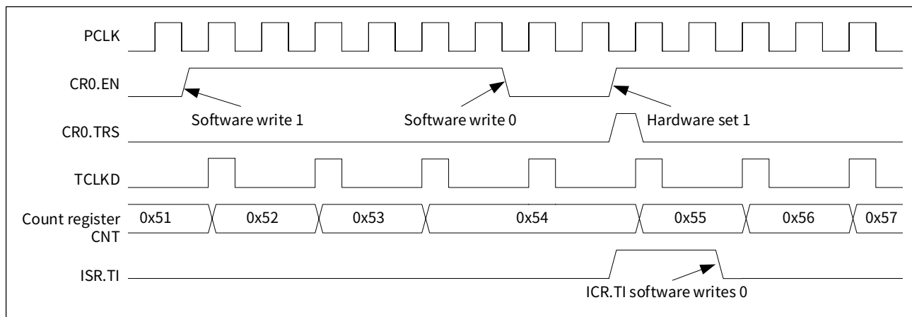
Figure 15-10 Timing diagram of trigger start mode (frequency division ratio is 2, PSC=0x01)
