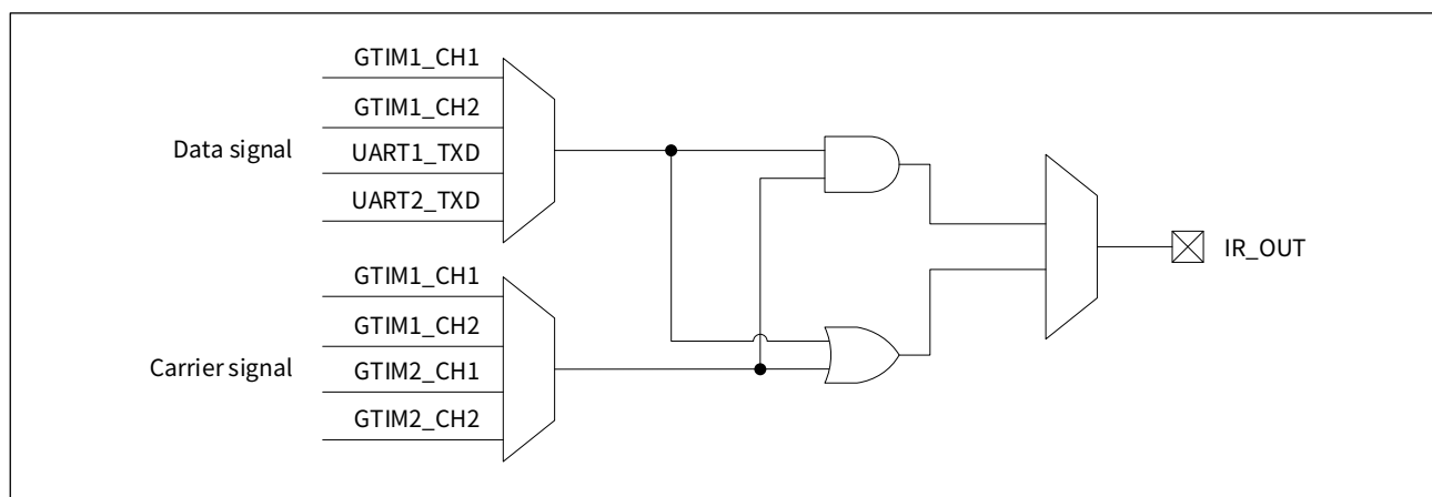
Figure 22-1 Schematic diagram of internal connection of IR
