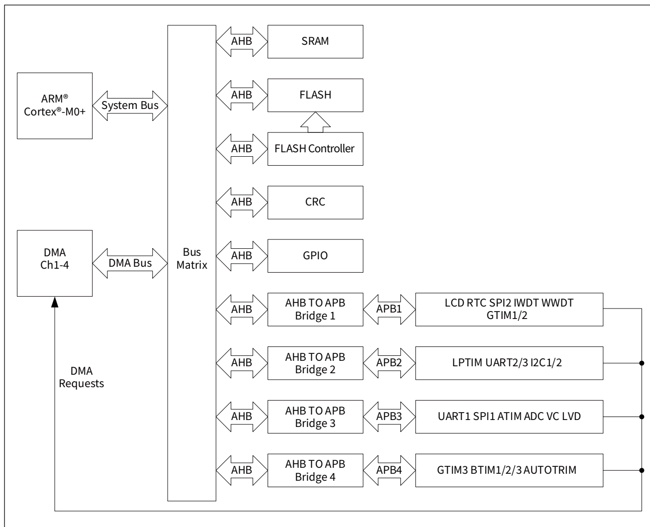
Figure 2-1 System architecture
