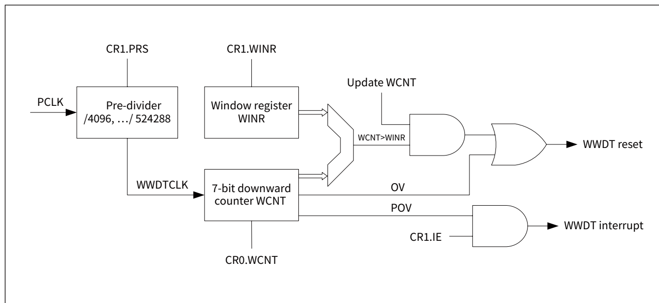
Figure 18-1 WWDT functional block diagram
