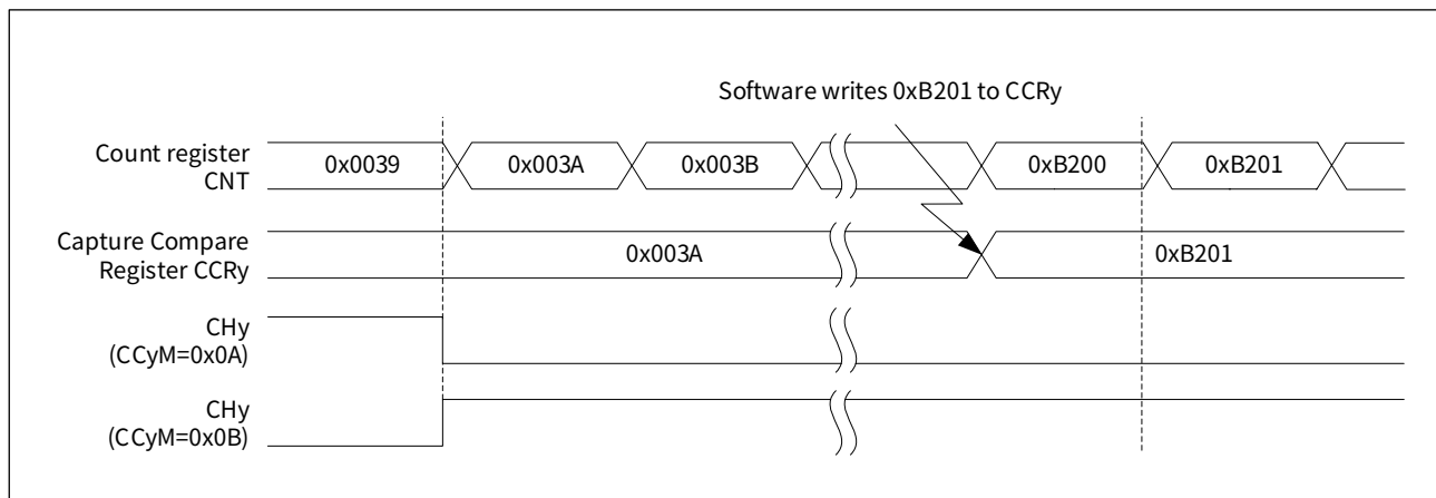
Figure 15-15 Two compare output modes
