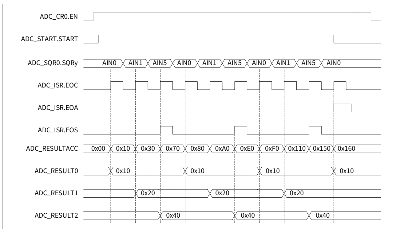
Figure 23-11 Accumulation conversion timing diagram
