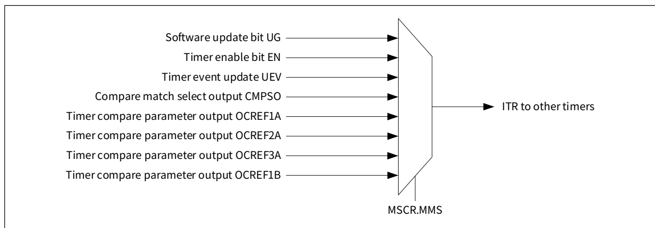
Figure 16-34 ATIM internal cascade ITR
