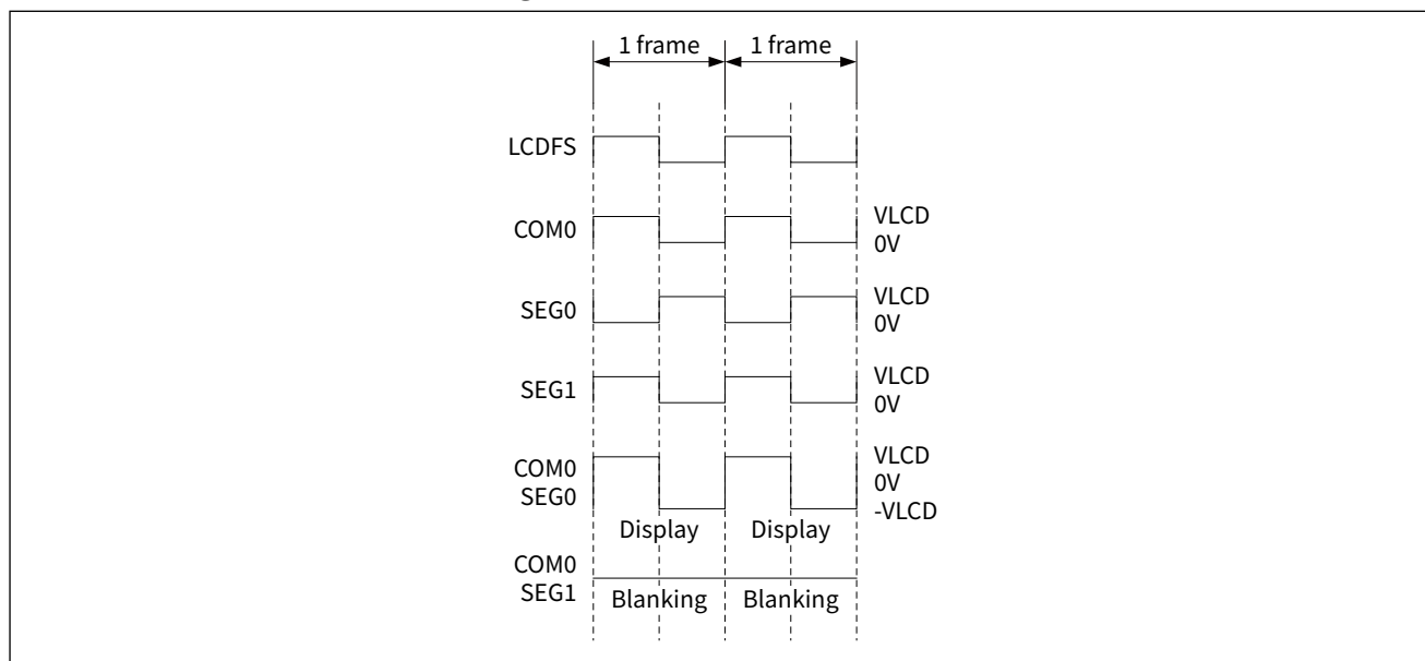
Figure 26-5 1/2 Duty 1/2 Bias driving waveform
