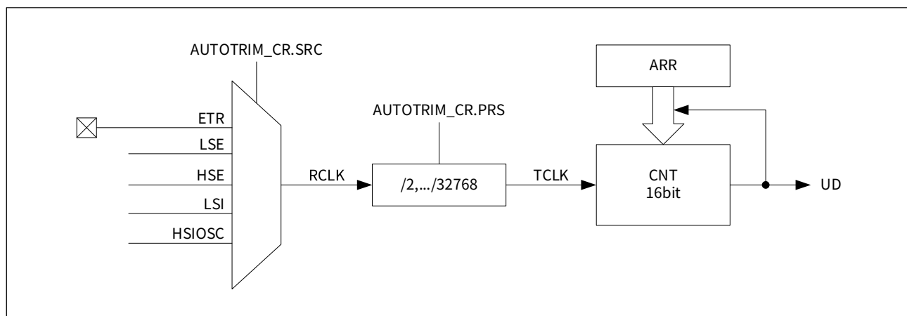
Figure 11-1 Automatic wake-up timer mode functional block diagram
