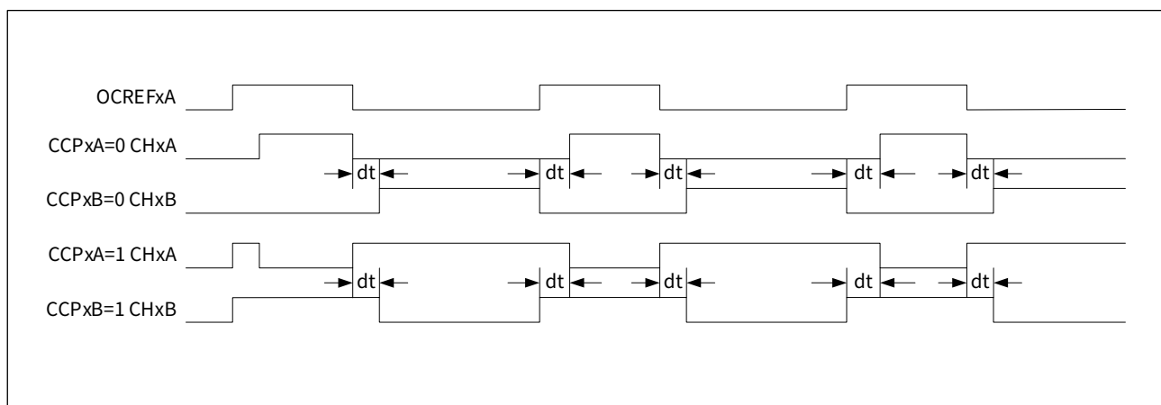
Figure 16-29 Complementary PWM output waveform with dead-time insertion
