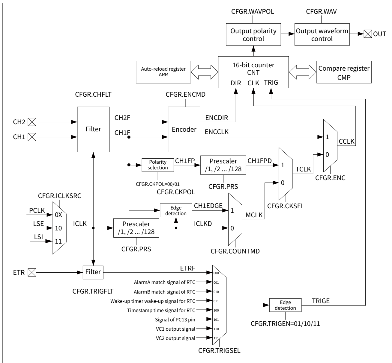
Figure 14-1 LPTIM functional block diagram
