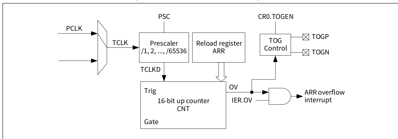
Figure 15-6 Timer mode block diagram
