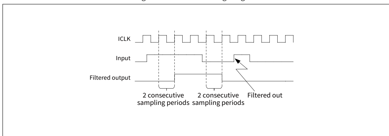
Figure 14-2 Filter Timing Diagram
