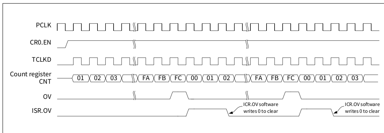
Figure 15-3 Continuous counting mode (PSC=0x00, ARR=0xFC)
