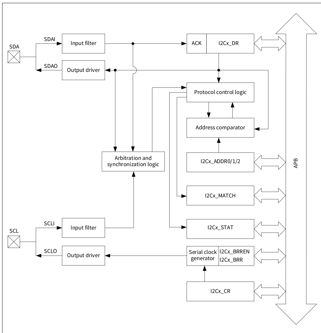
Figure 21-6 I2C functional block diagram
