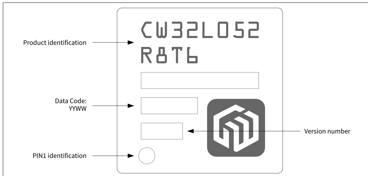
Figure 8-2 LQFP64 (10mm x 10mm) topside marking example
