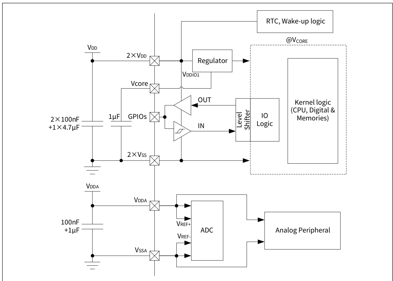
Figure 7-3 Power system
