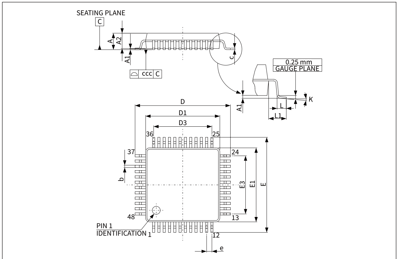
Figure 8-5 LQFP48 outline
