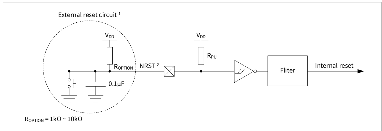
Figure 7-8 Recommended NRST pin protection
